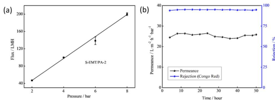
Fig. 11 (a) Water flux of the S-EMT/PA-2 membrane under different pressures. (b) Stability test of the S-EMT/PA-2 membrane at operating pressure of 3 bar and dye (Congo red) concentration of 50 ppm at room temperature.
