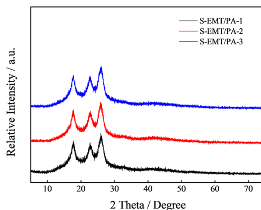
Fig. 5 XRD patterns of S-EMT/PA-1, S-EMT/PA-2 and S-EMT/PA-3 membranes.
