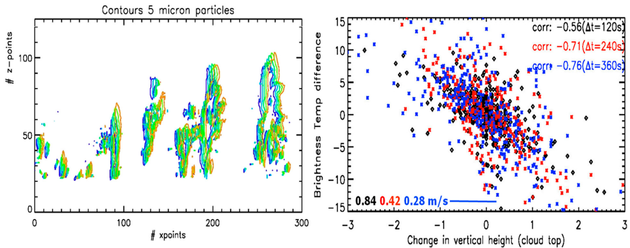
Fig. 4. Cloud-resolving model simulation at a horizontal grid of 200 m over 2–6 min. (left) Section in height and zonal ( u ) direction of the cloud boundaries as defined by the presence of 5- \mu\text{m} particles contoured at t = 0, 2, 4, 6, and 8 min. (right) Brightness temperature and height changes of simulated pixels with clouds over 2, 4, and 6 min; numbers in the bottom-left corner specify the unit vertical motion ( \text{m s}^{-1} ) for each time interval. Besides advection by the uniform large-scale wind ( u = 3.3 \text{ m s}^{-1} ), cloud transformation is evident on the minute scale. Credits: Gerd-Jan van Zadelhoff, KNMI.
