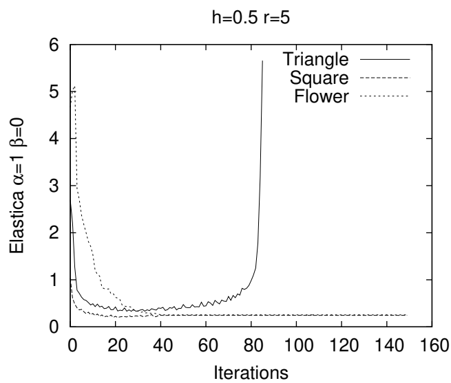
Fig. 6: The choice of radius impacts the flow. In the figures, the flow ceases to evolve for all shapes when r = 3 (a). In figure (b), for r = 5 , the triangle evolves to a single point, while the others stop in an intermediate shape, as in (a). In figure (c), we observe that for a given choice of radius, the elastica may increase after a certain number of iterations.
