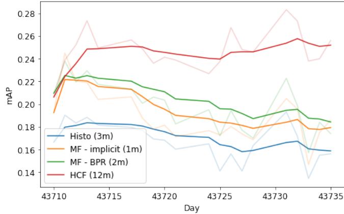
Figure 4: Daily evolution of symmetrized mAP during the test period. Light shades correspond to the true daily symmetrized mAP values, and dark ones to exponentially weighted averages ( \alpha = 0.2 ) of these values.
