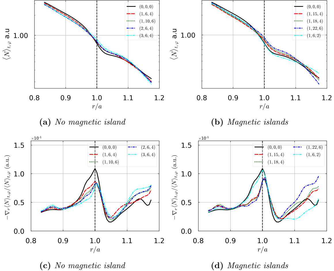
Figure 4: Radial profiles of the mean density (4a,4b) in log scale and of the density gradient length (4c,4d) at the LFS midplane for different magnetic perturbations (MPs). MPs with no magnetic island in the simulation box (4a,4c). MPs with magnetic islands (4b,4d). Quantities are averaged on time t and toroidal direction \varphi . The vertical dashed line is the separatrix.
