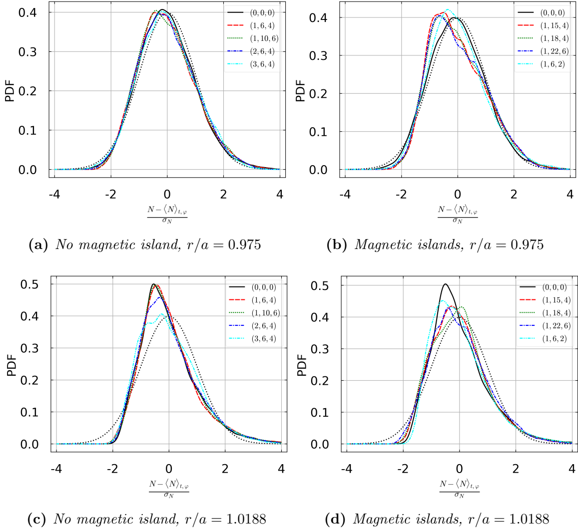
Figure 11: Normalized PDFs of density events along (t, \varphi) -axis at the LFS midplane and at two radial positions in the CFR and in the SOL, i.e. r/a = 0.98 (11a,11b) and r/a = 1.02 (11c,11d). Cases with no magnetic island (11a,11c) in the simulation box. Cases with magnetic islands (11b,11d). As a reference, the dotted black line corresponds to an exact Gaussian. The color zones is the histogram of each curve. The curves have been obtained with a kernel density estimation.
