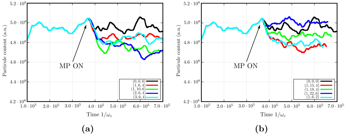
Figure 3: Time traces of the particle content in the simulation box for the case with magnetic islands outside the box (3a) and inside (3b).
