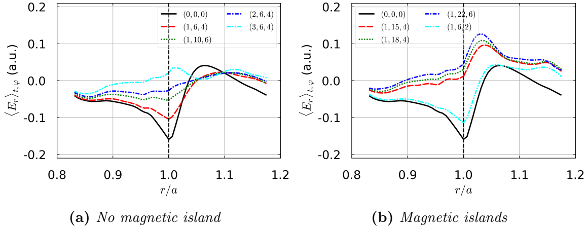
Figure 5: Radial profiles of the mean radial electric field E_r = \langle -\partial_r \Phi \rangle_{t,\varphi} (5a,5b) at the LFS midplane for different magnetic perturbations (MPs). MPs with no magnetic islands (5a) in the simulation box. MPs with magnetic islands (5b). Quantities are averaged on time t and toroidal direction \varphi . The vertical dashed line is the separatrix.
