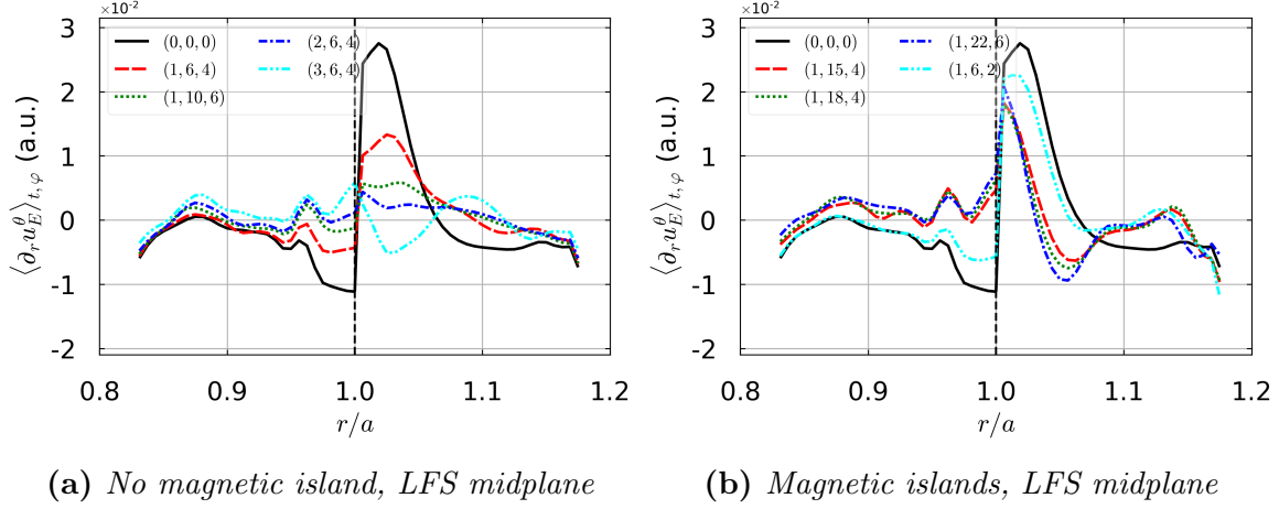
Figure 13: Radial profiles of the E \times B shear averaged over (t, \varphi) at the LFS midplane (13a,13b), \langle s_{E \times B} \rangle_{t,\varphi} = \langle \partial_r u_{E \times B}^\theta \rangle_{t,\varphi} . \langle s_{E \times B} \rangle_{t,\varphi} = \langle \partial_r u_{E \times B}^{\theta*} \rangle_{t,\varphi} . MPs corresponding to magnetic islands into the computational domain (13b) or not (13a)
