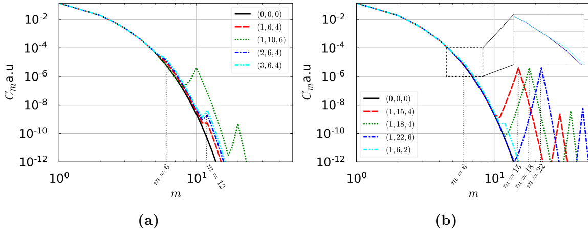
Figure 2: Fourier transform F_B of the amplitude of the magnetic field B in the poloidal direction, with m the poloidal wave number ( C_m = |F_B(m)| ). MPs without (2a) or with (2b) magnetic islands inside the computational domain. r/a = 0.9 and \varphi = \pi/8 .
