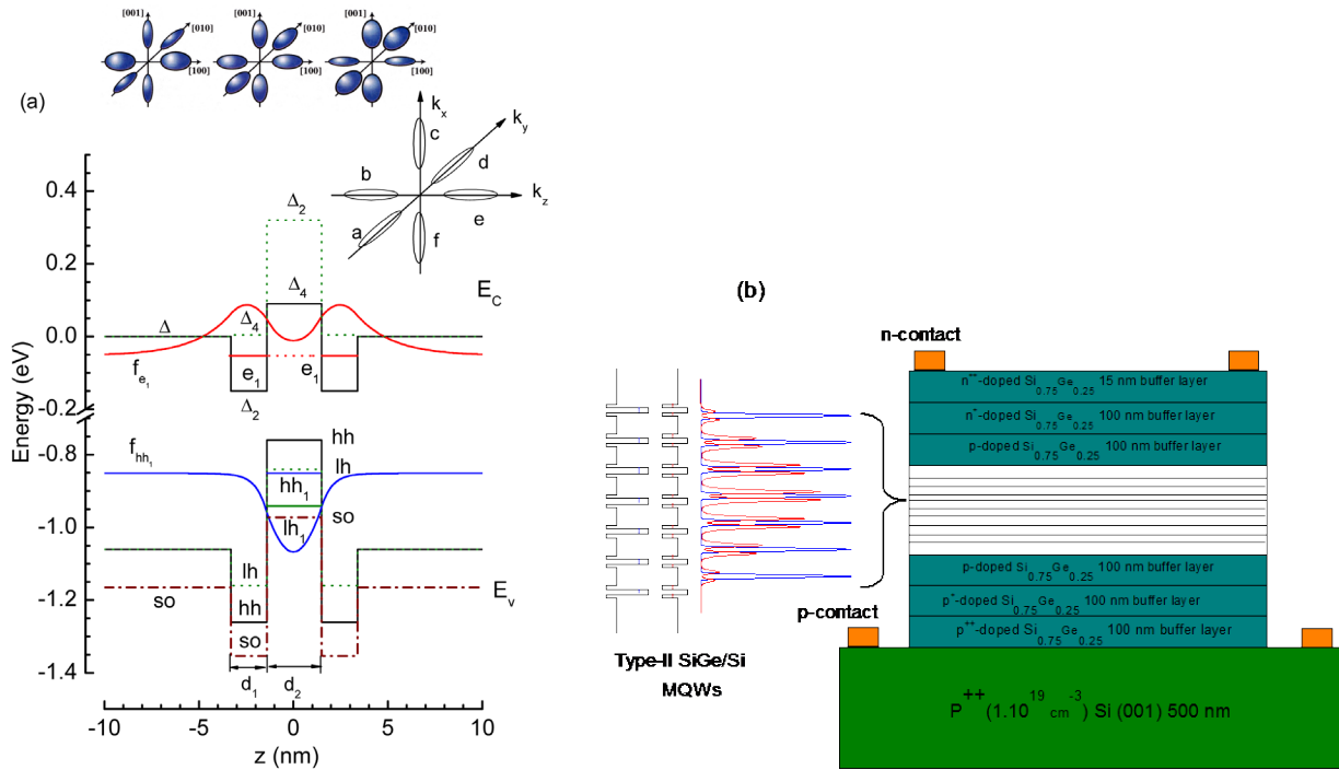
Figure 1. (a) Conduction and valence bands profile along the strained Si 1-y Ge y /Si/Si 1-x Ge x /Si/Si 1-y Ge y structure with strain-induced energy-split bands. In insert are shown the six iso-energetic ellipsoidal surfaces of conduction for unstrained Si 1-y Ge y ; (b) Schematic diagram of a p-i-n photodetectors. The cross-sectional view shows the structure of strained SiGe/Si W-multiple quantum wells grown on silicon on relaxed SiGe direct buffers.
