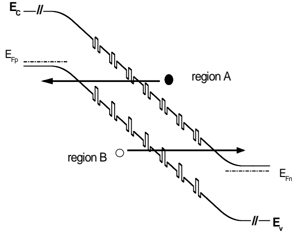
Figure 3. Energy band diagrams showing breakdown mechanisms of tunneling band to band in \text{Si}_{1-y}\text{Ge}_y/\text{Si}/\text{Si}_{1-x}\text{Ge}_x/\text{Si}/\text{Si}_{1-y}\text{Ge}_y MQW strain compensated photodetector device.
