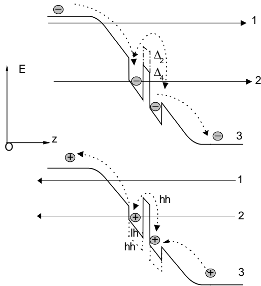
Figure 2. Energy band diagram of p-Si 1-y Ge y /Si 1-y Ge y /Si/Si 1-x Ge x /Si/Si 1-y Ge y /n-Si 1-y Ge y (y = 0.25, x = 0.60) stack under an external bias, and carrier behavior inside the structure: 1 is the tunneling transfer from extended states, 2 is the tunneling transfer from the localized states in pre-confinement region, and 3 is the thermally activated carrier transport.
