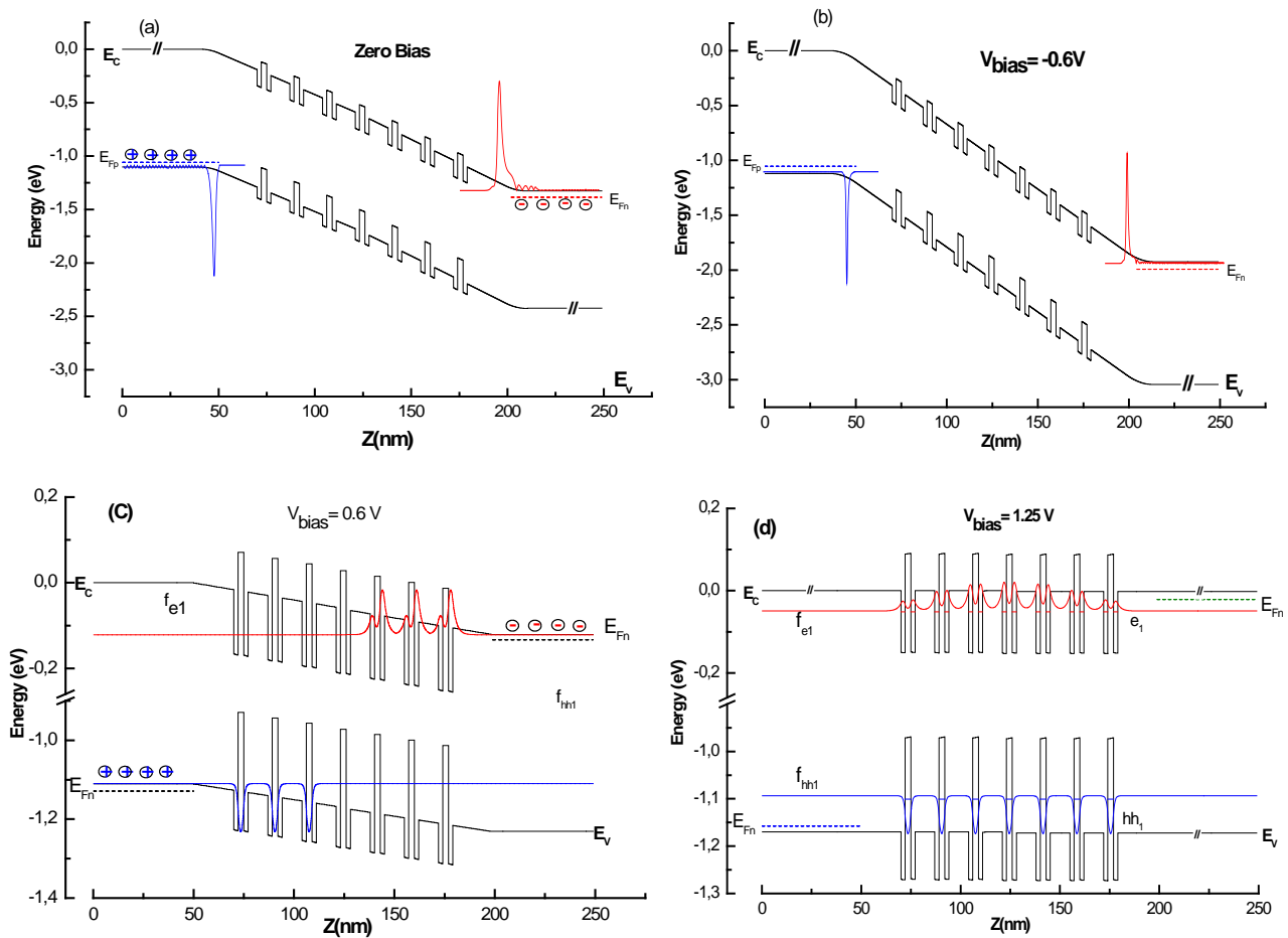
Figure 10. (a) Edges of the conduction and valence bands of the \text{Si}_{0.75}\text{Ge}_{0.25}/\text{Si}/\text{Si}_{0.4}\text{Ge}_{0.6}/\text{Si}/\text{Si}_{0.75}\text{Ge}_{0.25} MQW strain-compensated strained structures optimally designed for 1.55\ \mu\text{m} detection. The Fermi levels are drawn with their wave functions at zero bias; (b) Band diagram for a p-i-n photodetector under a reverse bias ( -0.6\text{V} ) at room temperature. E_{Fp} and E_{Fn} are the Fermi levels of conduction and valence bands; (c) The p-i-n heterojunction at direct bias ( +0.6\text{V} ) with the Fermi levels and wave functions; (d) The modeling heterostructure at the mode of the plat band under V_{\text{bias}} = 1.25\text{V} . The Fermi levels and the e_1 and hh_1 quantum levels are drawn with their relative wave functions.
