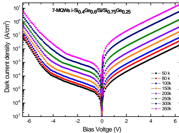
Figure 5. Dark current density of the p-i-n heterojunction based on Si 0.75 Ge 0.25 /Si 0.4 Ge 0.6 /Si 0.75 Ge 0.25 MQW strain-compensated strained structures of 100 \mu m in diameter versus bias voltage for temperatures from 50 to 350 K. The current is nearly symmetric to zero voltage.
