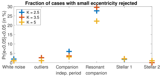
Figure 6. Fraction of cases where the posterior probability of e \in [0, 0.05] is below 0.05 for an injected circular signal and different noises described in Section 3.4.2. The blue, red, and yellow points correspond to the experiment for K = 2.5, 3.5, and 5 \text{ m s}^{-1} , respectively. The posterior distribution is computed with the model (24).
