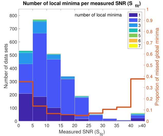
Figure B2. Blue bins: binned values of the number of systems with 1, 2, 3, 4, 5, 6, or 7 local minima, with a bin size in fitted SNR S_{\text{fit}} of 5. Red curve: fraction of the binned systems where the global minimum is not attained at the one obtained with a linear fit.
