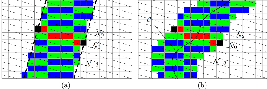
Fig. 2: (a) A directional scan in which the start scan S_0 in red, odd scans in green, even scans in blue, bounds of scan lines \mathcal{N}_i with dashed lines and bounds of scan strip \mathcal{D} with bold dashed lines. (b) An adaptive directional scan. The scan strip is dynamically fit to the curve position, and the scans are accordingly shifted to continuously cover the curve \mathcal{C} .
