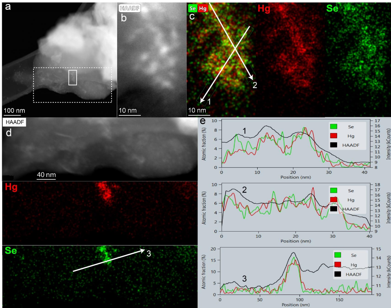
Figure S7. a) STEM-HAADF image of a liver region of petrel P4 rich in HgSeNP aggregates. b) Magnification of the (a) area framed with a plain line. c) EDX maps in fluorescence counts of Hg (red) and Se (green), and Hg-Se bi-color map of the (b) region. The arrows indicate the positions and directions of the EDX line profiles 1 and 2 shown in (e). d) Magnification of the (a) area framed with a dashed line (top), and
