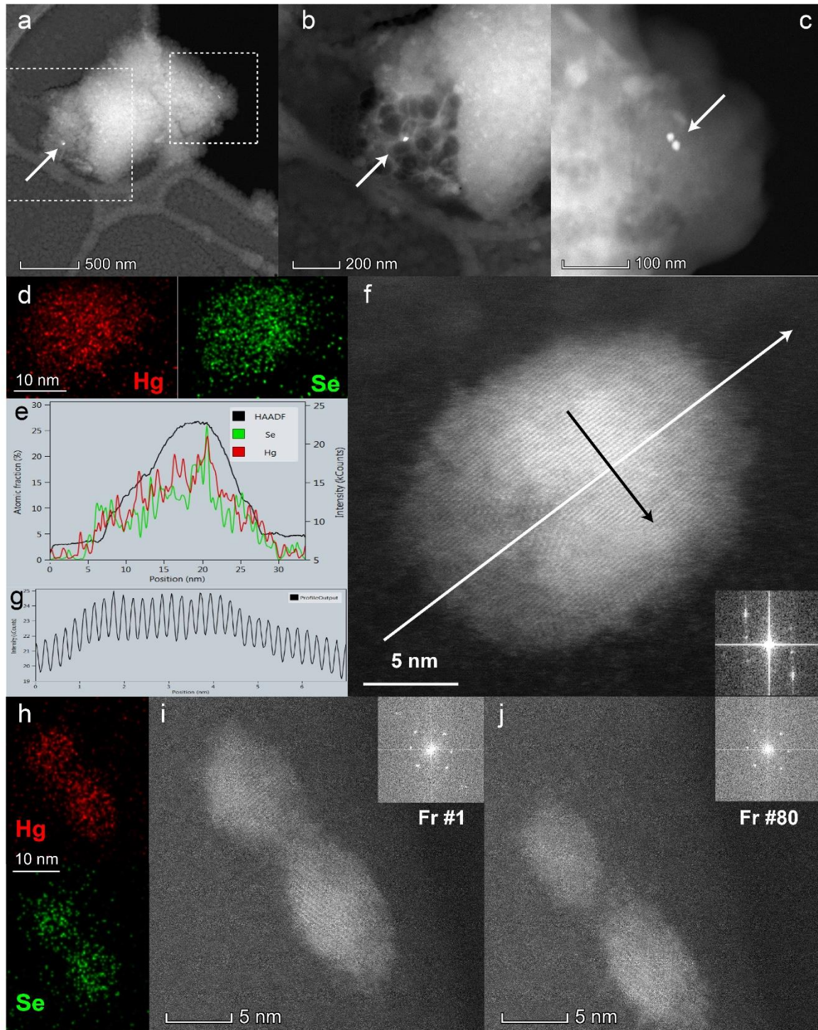
Figure S12. Small aggregates of \sim 30 nm HgSe NP and isolated 5 to 20 nm HgSe NP were imaged in the pectoral muscles of petrel P4, owing to the high scattering power of Hg and Se embedded in a thick and beam-sensitive organic matrix. a) STEM-HAADF image at -170^{\circ}\text{C} of a dried piece of muscle. b) HAADF image of the region pointed out with an arrow in (a) after degradation of the organic matrix under the electron beam. The HgSe grain was not altered under the beam, as confirmed by the HR-STEM contrast in (f). c) Magnification of the right framed area in (a) revealing two HgSe NP (same as those shown in Fig. 5c). d) EDX maps of Hg (red) and Se (green) from the HgSe NP pointed out in (c). e) Post-
