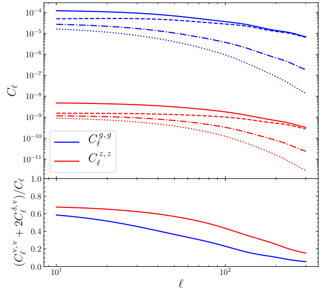
Fig. 2. Top panel: power spectra of angular galaxy clustering ( \delta_{\text{g}} , in blue) and ARF ( \delta_{\text{z}} , in red), for a Gaussian redshift bin taken in a DESI-like survey. The bin is centred on z_i = 0.75 and has a standard deviation of \sigma_z = 0.01 . The dashed line shows the term coming from the density kernel C_\ell^{\delta,\delta} , the dotted line shows the part coming from the velocity kernel C_\ell^{v,v} , and the dot-dashed line shows the cross term C_\ell^{\delta,v} . The total C_\ell power spectra (plain lines) correspond to the sum C_\ell = C_\ell^{\delta,\delta} + 2C_\ell^{\delta,v} + C_\ell^{v,v} . Bottom panel: velocity dependence ratio in the power spectrum (C_\ell^{v,v} + 2C_\ell^{\delta,v})/C_\ell over the complete power spectrum, for the angular galaxy clustering (blue line) and for the ARF (red line). This figure shows that ARF are more sensitive to the peculiar velocity of galaxies than angular galaxy clustering, for the same redshift shell.
