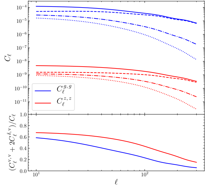
Fig. 2. Top panel: power spectra of angular galaxy clustering ( \delta_{\text{g}} , in blue) and ARF ( \delta_z , in red), for a Gaussian redshift bin taken in a DESI-like survey. The bin is centred on z_i = 0.75 and has a standard deviation of \sigma_z = 0.01 . The dashed line shows the term coming from the density kernel C_\ell^{\delta,\delta} , the dotted line shows the part coming from the velocity kernel C_\ell^{v,v} , and the dot-dashed line shows the cross term C_\ell^{\delta,v} . The total C_\ell power spectra (plain lines) correspond to the sum C_\ell = C_\ell^{\delta,\delta} + 2C_\ell^{\delta,v} + C_\ell^{v,v} . Bottom panel: velocity dependence ratio in the power spectrum (C_\ell^{v,v} + 2C_\ell^{\delta,v})/C_\ell over the complete power spectrum, for the angular galaxy clustering (blue line) and for the ARF (red line). This figure shows that ARF are more sensitive to the peculiar velocity of galaxies than angular galaxy clustering, for the same redshift shell.
