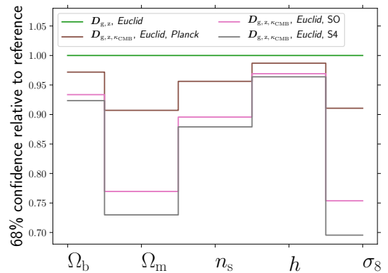
Fig. 10. Ratio of 1\sigma constraints for \Lambda CDM parameters from D_{g,z,KCMB} over the 1\sigma constraints from D_{g,z} for the Euclid -like spectroscopic survey. We show combinations with CMB lensing from Planck (brown), the Simons Observatory (pink), and CMB-S4 (grey). Constraints are marginalised over the 20 galaxy bias parameters.
