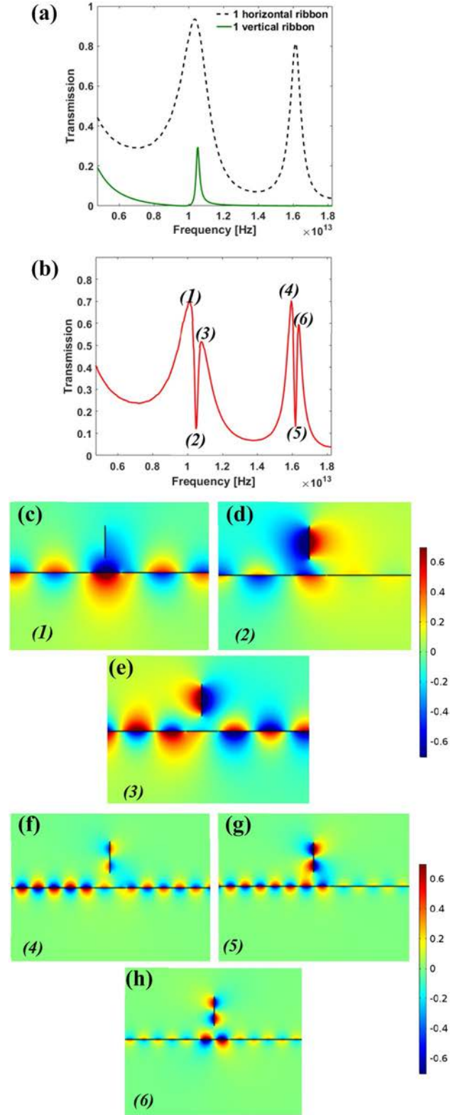
Fig. 9 a Transmission spectrum of the structure of Fig. 1b when a single ribbon is coupled to the waveguide with l_1 = 250 nm and g = 10 nm for the horizontal ribbon (black curve). For the ribbon shifted above the waveguide (green curve), the parameters are: l_2 = 250 nm, d = 120 nm and \theta = 0^\circ . The Fermi energy level of the ribbons is E_{F1} = 160 meV. b Same as in a but when both ribbons are present in the structure. c–h z -component of the magnetic field map at the transmission dips and peaks frequencies labeled (1)–(6), in b , respectively
