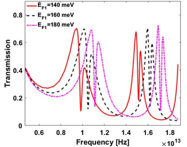
Fig. 13 Transmission spectra of the system for different values of E_{F1} . Remaining parameters are the same as in Fig. 8b
