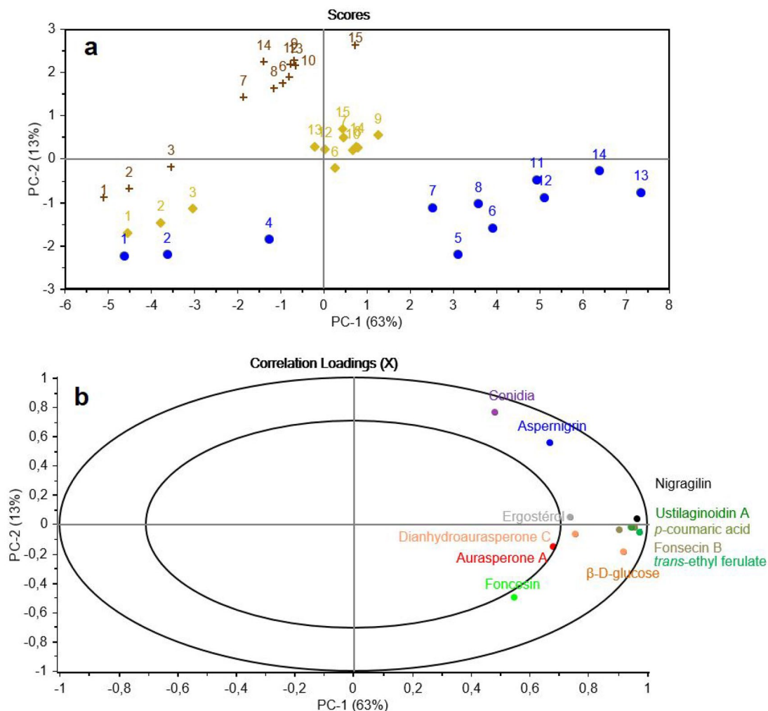
Fig. 5 PCA of the metabolic production related to the moisture content variations (plus 50% diamond 60% circle 66%) in the (PC1, PC2) plane: score plot (a) and correlation loadings (b) (color figure online)
