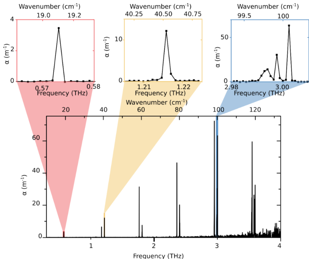
Figure S 2: Experimental spectrum of the absorbance of 10 mbar gaseous NH 3 from our experiments (simple FFT) showing that the spectrum extends from 200 GHz to 4 THz with narrow lines distributed from 500 z to 3.6 THz. It was recorded using the 7 cm long Brewster angle gas cell in the TDS setup. The three top insets shows a zoom on the lines studied in the paper.
