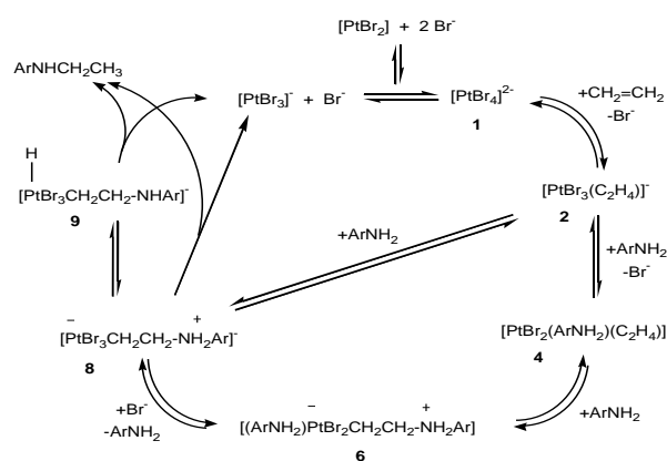
Scheme 1. Proposed 3 “productive” mechanism for the hydroamination of ethylene by aniline.
