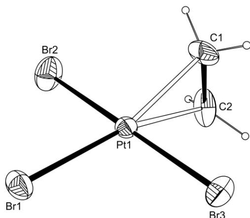
Figure 1. Molecular structure of anion of 2 with ellipsoids are drawn at the 30% probability level. Selected bond distances (Å): Pt-Br1, 2.4294(14); Pt-Br2, 2.4229(16); Pt-Br3, 2.4337(14); C1-C2, 1.37(2).
