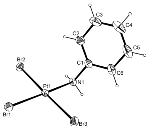
Figure 2. Molecular structure of the anion of 3 with molecular ellipsoids are drawn at the 30% probability level. Selected distances (Å): Pt-Br1, 2.4444(9); Pt-Br2, 2.4487(7); Pt-Br3, 2.4375(7), Pt-N1, 2.078(4).
