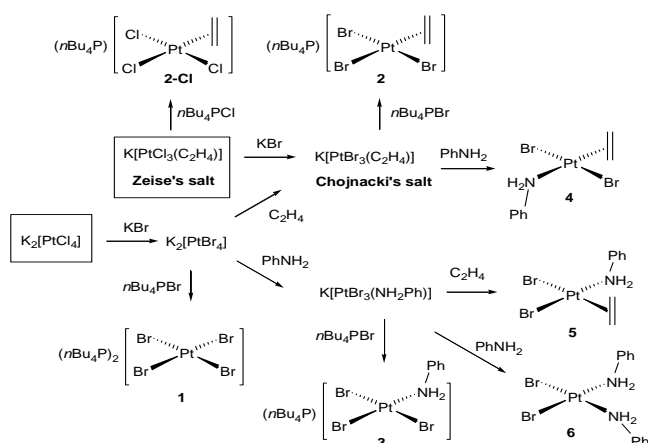
Scheme 2. Synthesis of bromoplatinum(II) complexes in “one-pot” procedures from K_2PtCl_4 or Zeise’s salt.
