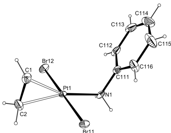
Figure 3. An ORTEP view of one of the two independent molecules of 4 . Molecular ellipsoids are drawn at the 30% probability level. Selected bond distances (Å; values separated by slashes are the corresponding parameters in two crystallographically independent molecules): Pt1-Br11, 2.4108(6)/2.4093(7); Pt1-Br12, 2.4203(6)/2.4237(7); Pt1-N1, 2.093(4)/2.093(5); Pt1-C1, 2.155(6)/2.158(7); Pt1-C2, 2.145(6)/2.153(6); C1-C2, 1.378(10)/1.375(9).
