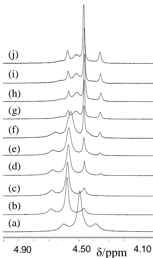
Figure 8. ^1\text{H} NMR spectra in \text{DMF-}d_7 at 298K of: 5 (a); 5 + n\text{Bu}_4\text{PBr} (0.87 equiv) at 0 (b), 10 (c), 50 (d), 107 (e), 257 min (f); 21.5 (g) 24 (h), 28 (i), and 48 h (j).
