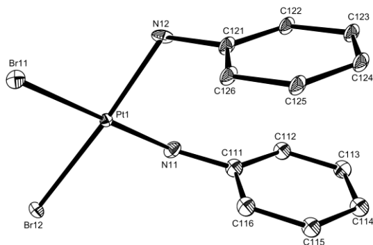
Figure 6. An ORTEP view of one of compound 6 . Molecular ellipsoids are drawn at the 30% probability level.
