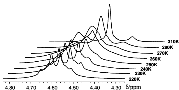
Figure 4. Variable temperature 1 H NMR spectrum of 5 in DMF- d 7 .
