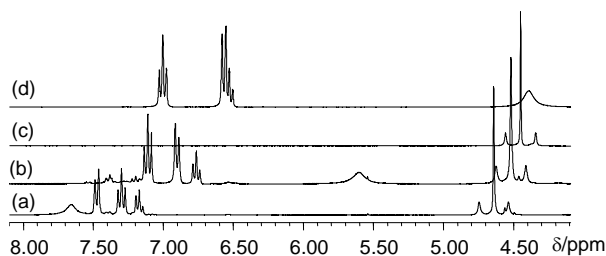
Figure 7. ^1\text{H} NMR spectra (olefin, \text{NH}_2 and aromatic-region) of: a) 4 ; b) 4 in the presence of 0.72 equiv n\text{Bu}_4\text{PBr} ; c) 2 ; and d) aniline, in \text{THF-}d_8 at 298K. [\mathbf{4}] = [\mathbf{2}] = 0.5 \cdot [\text{PhNH}_2] = 0.04 \text{ M} .
