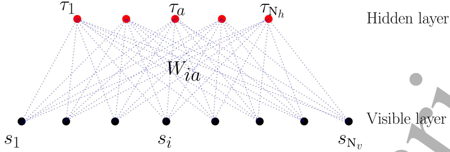
Fig. 1. Bipartite structure of the RBM.
