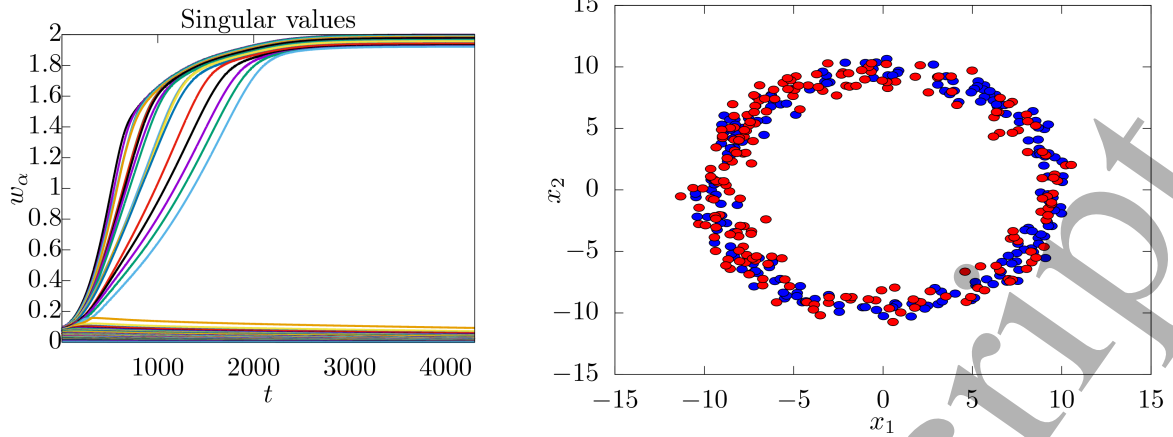
Fig. 6. Left: the learning curves for the modes w_\alpha using an RBM with (N_v, N_h) = (100, 100) learned on a synthetic dataset distributed in the neighborhood of a 20d ellipsoid embedded into a 100d space. Here the modes interact together: the weaker modes push the stronger ones higher, and they all accumulate at the top of the spectrum, as explained in Section 3.2. Right: a scatter plot projected on the first two SVD modes of the training (blue) and sampled data from the learned RBM (red) for a problem in dimension N_v = 50 with two condensed modes. We can see that the learned matrix \mathbf{u} captures relevant directions and that the RBM generates data perfectly similar to the one of the training set.
