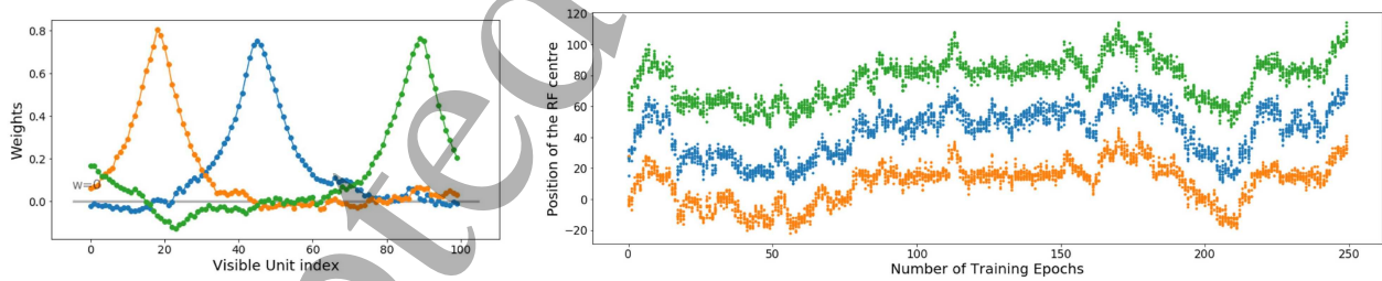
Fig. 7. Left: figure from Ref. [68], the value of w_i for each visible site of a RBM with 3 hidden nodes trained on the dataset of the 1D homogeneous Ising model with periodic boundary condition. We see three similarly peak shaped potentials with a decreasing magnitude of similar order for the three. Each peak intends to reproduce the correlation pattern around a central node, and therefore cannot reproduce the translational symmetry of the problem. Right: figure from Ref. [68], the position of the three peaks as a function of the number of training epochs. We observe that the peaks diffuse while repelling each others. The diffusion aims at reproducing the correlation patterns of the translational symmetry, while the repelling interaction ensure that two peaks will not overlap..
