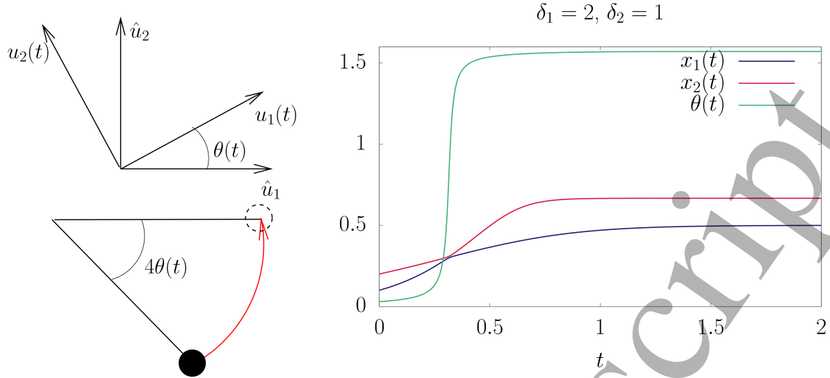
Fig. 2. Angle between the reference basis given by the data and the moving one given by the RBM shown on the up left panel. Equivalence with the motion of a pendulum is indicated on the left bottom panel. Solution of (18,19,20) of two coupled modes in the linear RBM (right panel).
