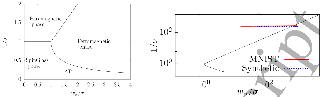
Fig. 4. Left: the phase diagram of the model. The y-axis corresponds to the variance of the noise matrix, the x-axis to the value of the strongest mode of w . We see that the ferromagnetic phase is characterized by having strong mode eigenvalues. In this phase, the system can behave either by recalling one eigenmode of w or by composing many modes together (compositional phase). For the sake of completeness, we indicate the AT region where the replica symmetric solution is unstable, but for practical purpose we are not interested in this phase. Right: An example of a learning trajectory on the MNIST dataset (in red) and on a synthetic dataset (in blue). It shows that starting from the paramagnetic phase, the learning dynamics brings the system toward the ferromagnetic phase by learning a few strong modes.
