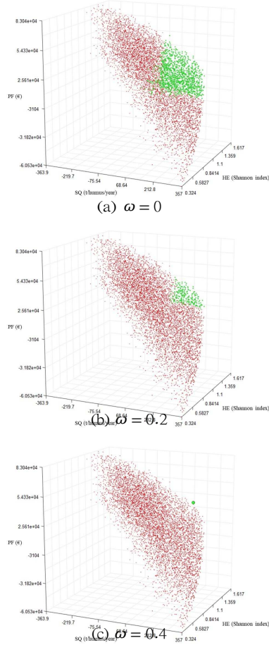
Figure 6: The three-dimensional scores (soil quality SQ, heterogeneity HE and profit PF) of non-viable and viable scenarios (in red and green, respectively) for different values of \omega .
