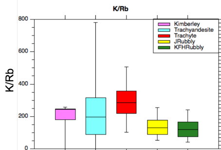
Fig. 2: K/Rb ratio for the Kimberley sediments enriched in sanidine, trachyandesite/plagioclase and trachyte/orthoclase, and for the Rubbly bedrock of Jura member.
