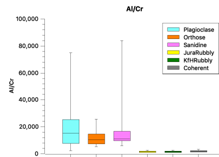
Fig. 4: Al/Cr ratio distribution in the feldspars (Plagioclase, Orthose and Sanidine) and in the Rubbly (Jura and KHm) and Coherent bedrock.
