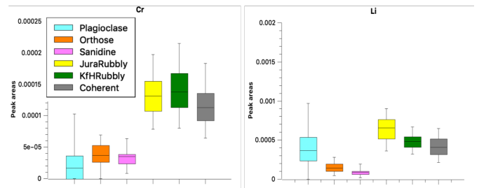
Fig. 3: Cr (left) and Li (right) peak areas distribution in the feldspars (Plagioclase, Orthose and Sanidine) and in the Rubbly (Jura and KHm) and Coherent bedrock.
