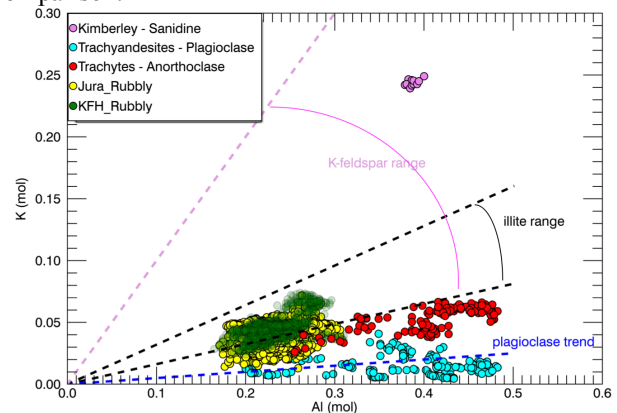
Fig. 1: K vs Al (mol) for the GT Rubbly bedrock along with feldspars seen along the traverse. Each data point corresponds to a single laser shot. The dashed lines correspond to the theoretical trend for plagioclase (blue), sanidine (pink), with K-feldspar (pink) and illite (black) ranges.
