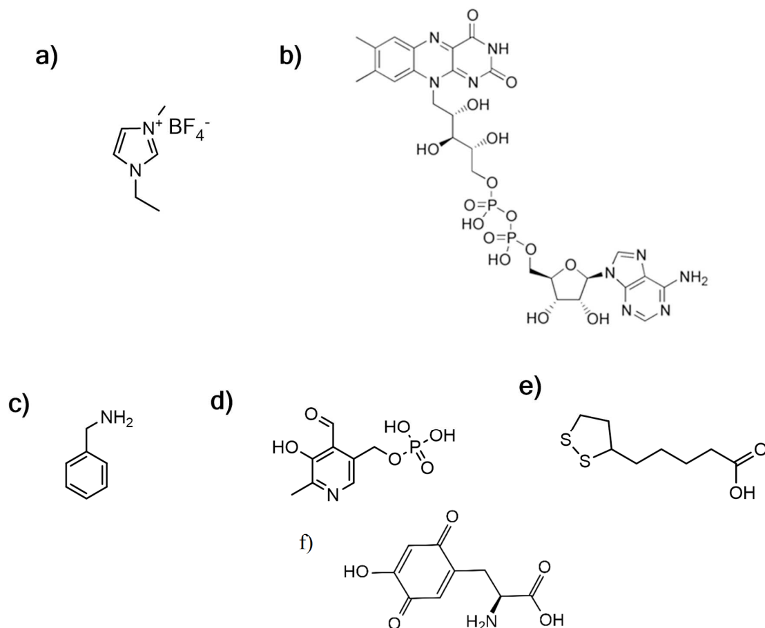
Figure 2. (a) 1-Ethyl-3-methylimidazolium tetrafluoroborate (emimBF 4 ); (b) flavin adenine dinucleotide (FAD); (c) benzylamine; (d) pyridoxal phosphate (PLP); (e) α-lipoic acid (LA), (f) topoquinone (TPQ)
