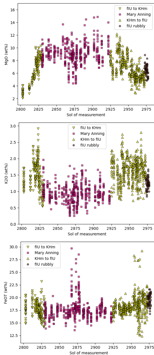
▲ Figure 2: variations in MgO, K 2 O and FeO T abundances (wt%) along the traverse. The x axis shows time of measurement and does not reflect horizontal distance. The diagrams start just after the departure from Bloodstone Hill and ends at the Sands of Forvie (see Figure 1 for localization of the rover stops). Each symbol corresponds to a single LIBS point on a bedrock target, excluding Ca-sulfate veins and soils.
