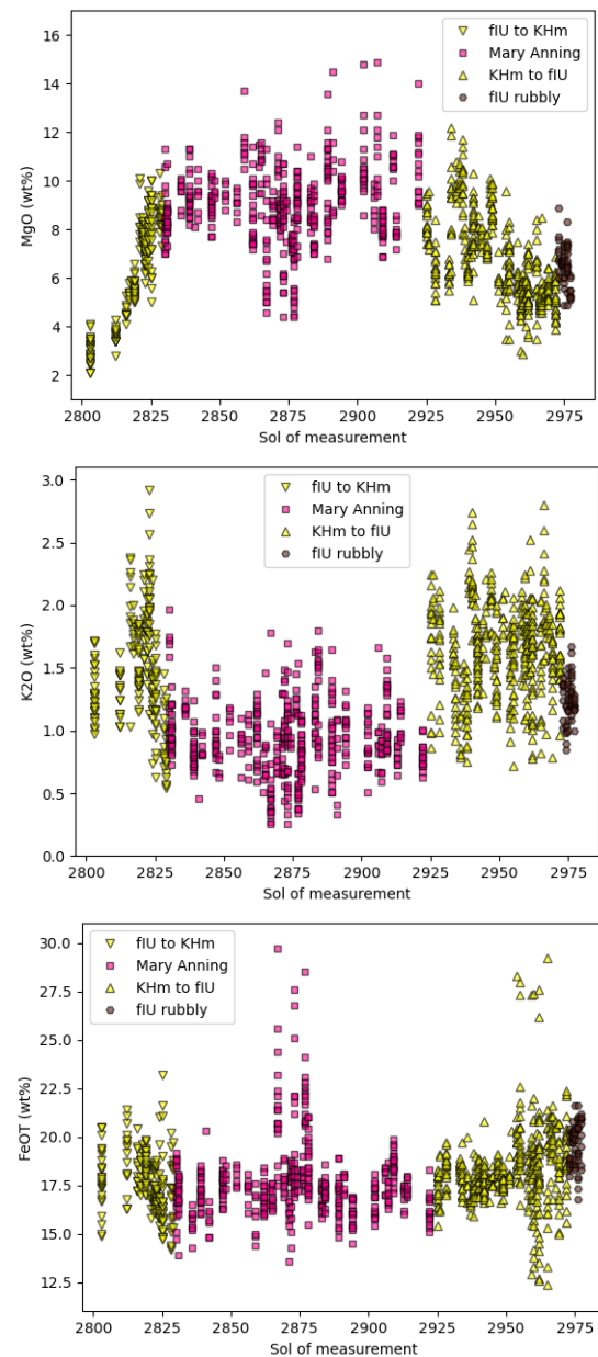
▲ Figure 2: variations in MgO, K 2 O and FeO T abundances (wt%) along the traverse. The x axis shows time of measurement and does not reflect horizontal distance. The diagrams start just after the departure from Bloodstone Hill and ends at the Sands of Forvie (see Figure 1 for localization of the rover stops). Each symbol corresponds to a single LIBS point on a bedrock target, excluding Ca-sulfate veins and soils.
