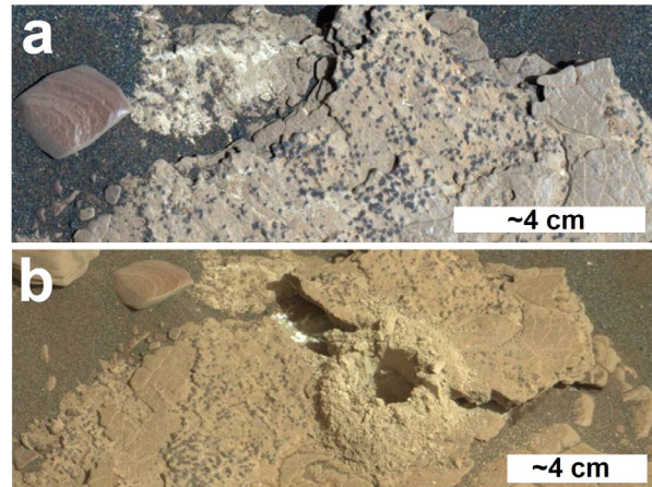
Fig. 1. (a) Groken target with dark-toned nodules (MAHLI 2906MH000240011003483C00). (b) After drilling, the Groken slab fractured and exposed a bright-toned Ca-sulfate vein (Mastcam 2910MR0151870011300451E01).
