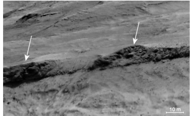
Fig. 6: The erosion-resistant lip identified as a “Marker Bed” transition (~9 km away).
