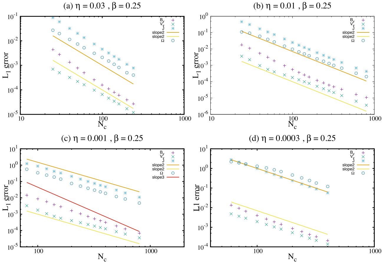
Figure 9. Error convergence for the reconnective diffusion problem. L_1 error on B_x , V_y , J , and \Omega , as a function of the number of grid cells N_c in each direction. The linear (slope 1), parabolic (slope 2), and cubic (slope 3) convergence orders are also indicated with plain line. Optimal 2\pi/L_x values of 2, 3, 10, and 30 are used for \eta = 0.03 (a), \eta = 0.01 (b), \eta = 0.001 (c), and \eta = 0.0003 (d), respectively. A non-uniform cell spacing in x -direction is used for \eta = 0.0003 case.
