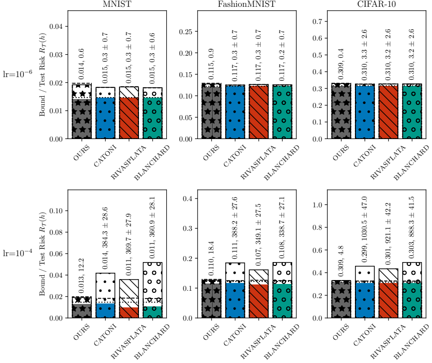
Fig. 4: The value of the bounds (hatched bars) and the test risks (colored bars) for Corollary 6 (“ours”) and Corollary 7 (“CATONI”, “RIVASPLATA” and “BLANCHARD”) in two different settings, i.e. , with a learning rate of 10^{-6} and 10^{-4} and with split ratio of 0.5. We also plot the value of the bounds (the dashed lines) and the test risks (the dotted lines) before executing Step 2) of our Training Method. The y-axis shows the values of the bounds and the test risks R_T(h) . The empirical risk R_S(h) is presented above each bar. Moreover, the second value represents the mean value of the divergence (the standard deviations are also given for the disintegrated bounds of the literature).
