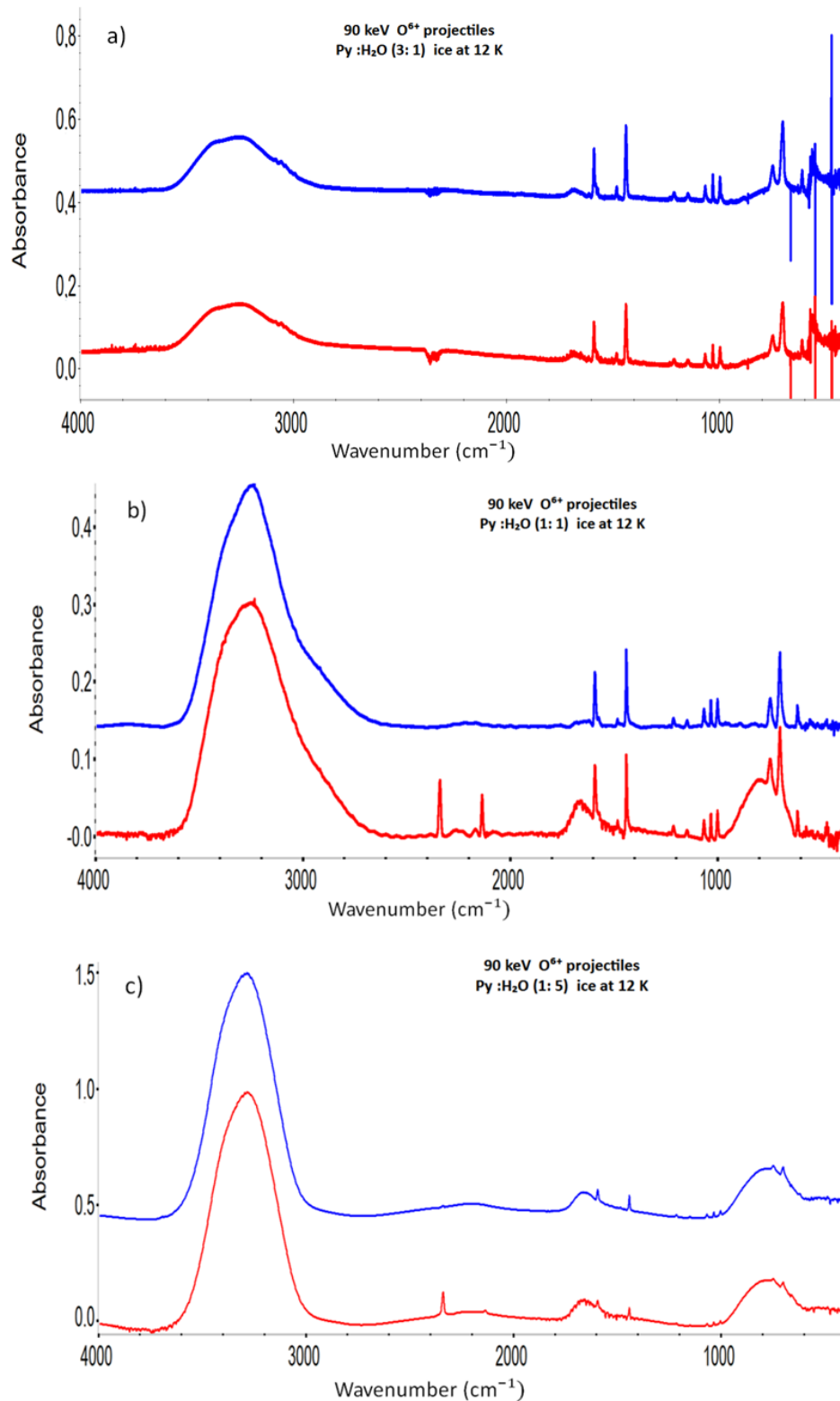
Fig. 6: FTIR spectra of (a) Py:H 2 O (3:1) ice before (upper line) and after irradiation with a fluence of 8 \times 10^{14} ions \text{cm}^{-2} (bottom line), of (b) Py:H 2 O (1:1) ice before (upper line) and after irradiation with a fluence of 2.12 \times 10^{15} ions \text{cm}^{-2} and of (c) Py:H 2 O (1:5) ice before (upper line) and after irradiation with a fluence of 1.4 \times 10^{15} ions \text{cm}^{-2} (bottom line) by O 6+ (90 keV) beams at 12K. Spectra “before irradiation” were slightly shifted on the absorbance axis for better visibility.
