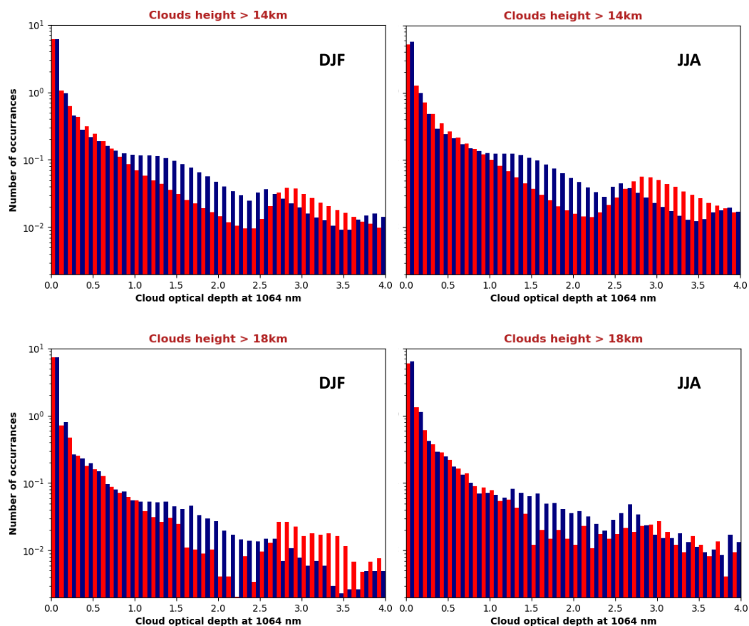
Figure 5. Normalized histograms of cloud optical depth (COD) for integrated high clouds at altitudes higher than 14 and 18 km from CATS (red bars) and CALIOP (blue bars) for DJF (left column) and JJA (right column). Note the logarithmic vertical scale.
