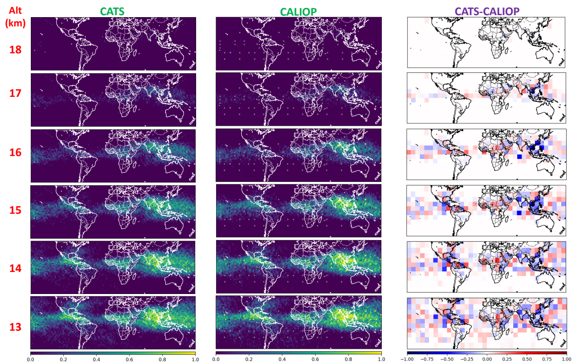
Figure 3. Same as Figure 2 but during JJA.
