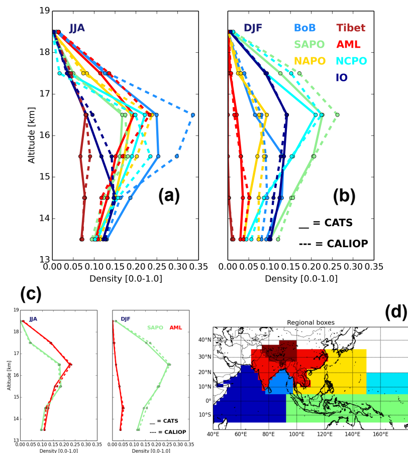
Figure 4. Vertical distribution of cloud density from CATS (solid lines) and CALIOP (dashed lines), in the altitude range 13–18 km for JJA (a) and DJF (b). Same as (a,b) but with CATS data temporally collocated with CALIOP overpasses, for selected regions (c). The seven subregions indicated in (d) are individuated with corresponding colors. A description of acronyms follows. IO: Indian Ocean, AML: Asian MainLand, Tibet: Tibetan Plateau, BoB: Bay of Bengal, NAPO: North Asian Pacific Ocean, SAPO: South Asian Pacific Ocean, NCPO: North Central Pacific Ocean.
