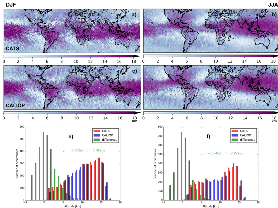
Figure 1. Mean maximum altitude of cloud top from Cloud–Aerosol Transport System (CATS) (a,b) and Cloud–Aerosol Lidar with Orthogonal Polarization (CALIOP) (c,d), years 2015–2016, day and night overpasses, for December–January–February (DJF) (a,c) and June–July–August (JJA) (b,d). Histogram of CATS and CALIOP maximum altitude of cloud top and their differences (CATS–CALIOP) for DJF (e) and JJA (f).
