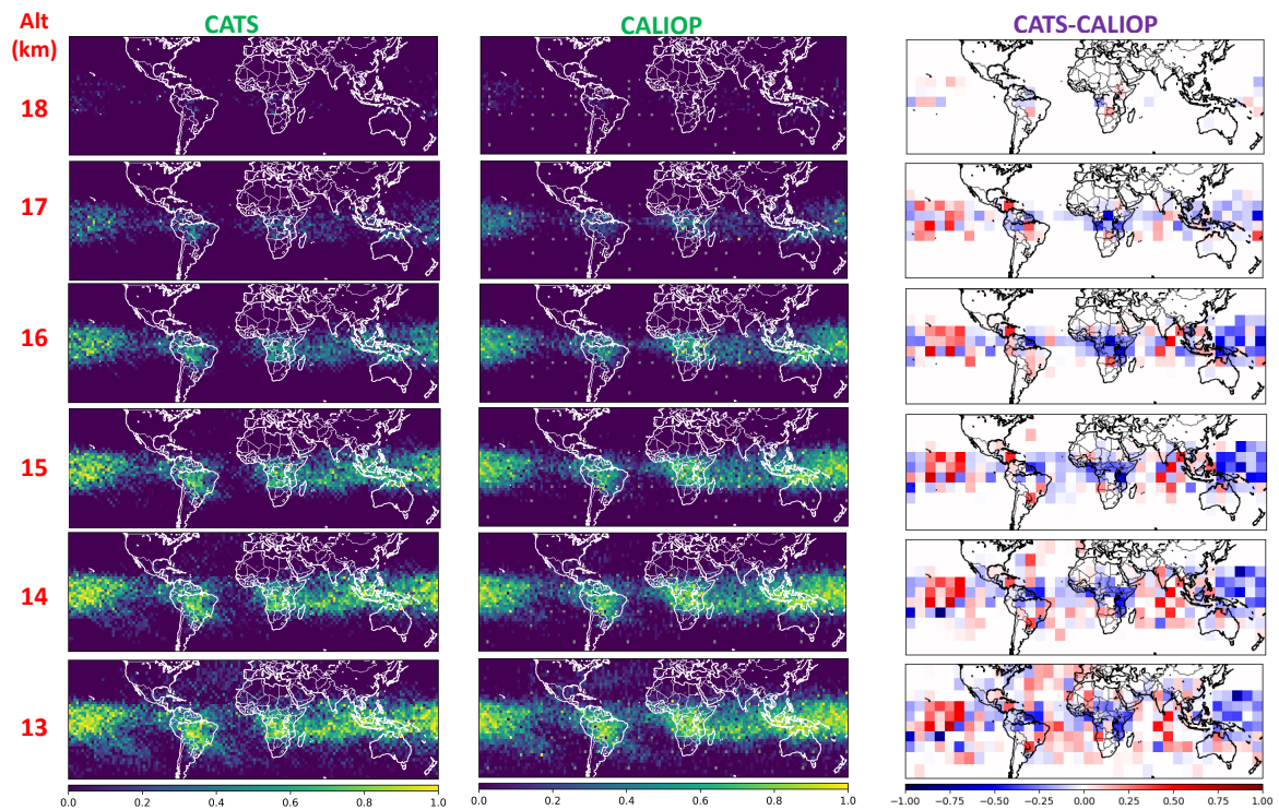
Figure 2. Global distribution of high clouds density from CATS (left column) and CALIOP (central column), years 2015–2016, day and night overpasses, during DJF. The CATS–CALIOP differences (based on a coarser 10^\circ \times 10^\circ grid) are shown as well (right column). The partial cloud covers and the differences are shown for top altitudes from 18 to 13 km (different rows).
