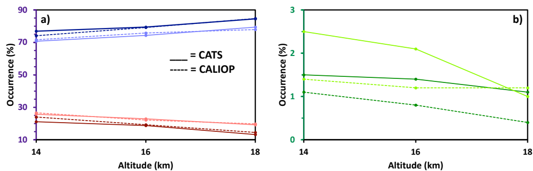
Figure 6. Percent occurrence of COD smaller than 0.3 (thin clouds, blue lines, left vertical scale), within the interval 0.3–3.0 (thick clouds, red lines, left vertical scale) (a) and bigger than 3.0 (very thick clouds, green lines, right vertical scale) (b), from CATS (solid lines) and CALIOP (dotted lines) for DJF (dark-colored lines) and JJA (light-colored lines).
