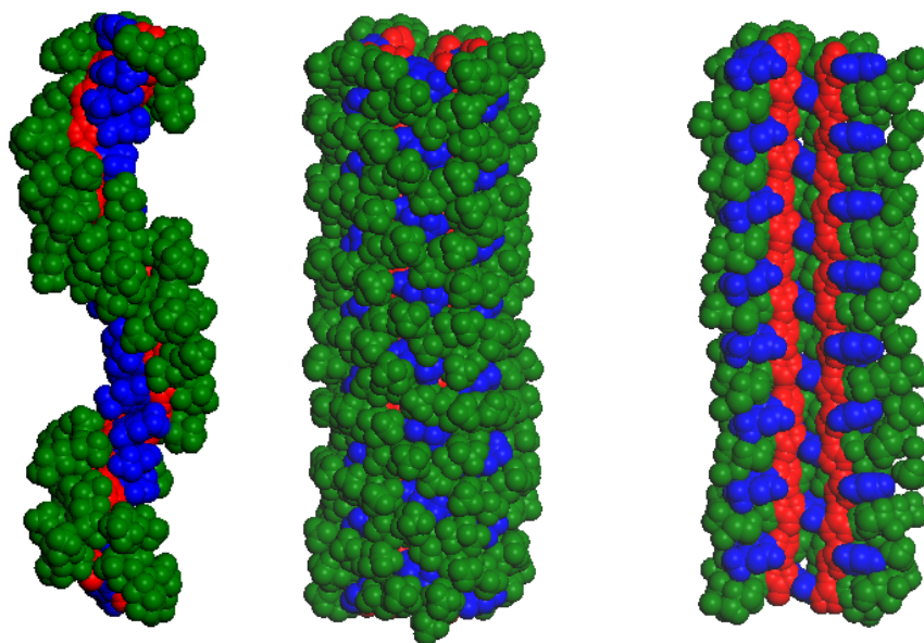
Figure 5. Pieces of filament (left), tube (center), and tube longitudinally cut in two to expose its inner part (right). The assemblies are of the same length (72 Å); the atoms are rendered as spheres having the Van der Waals radius of the elements (CPK representation). The urea moieties are in red, the toluene cores in blue, and the alkyl chains in green.
