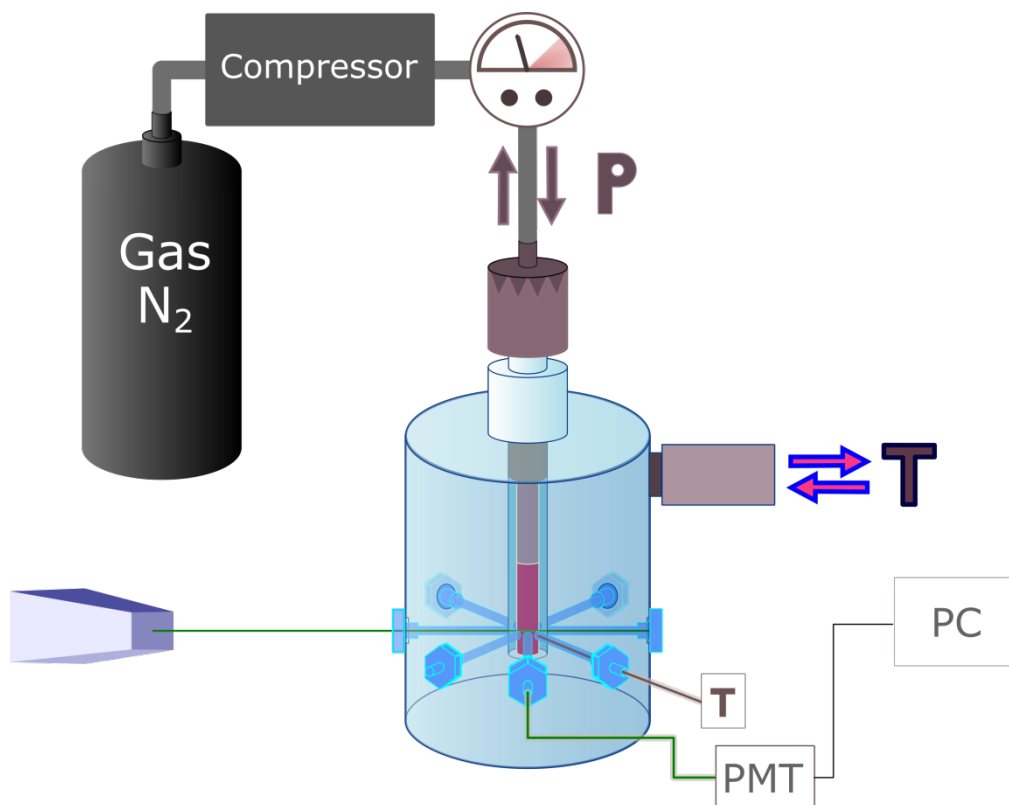
Figure 1: Schematic illustration of the experimental high-pressure DLS setup. Shown, out of scale, are: the gas (nitrogen) tank, compressor, chamber cell with different glass windows for scattering at different fixed angles, gas inlet to DLS cell (P), inlet of recirculating fluid to cell chamber for maintaining constant temperature (T with arrows), temperature meter (T), laser (with green incident beam), scattered beam entering the photomultiplier tube (PMT), whose signal is collected and analyzed by a correlator on a PC.
