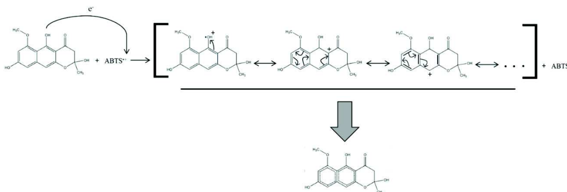
Figure 4. Radical scavenging mechanism of the fonsesic.
