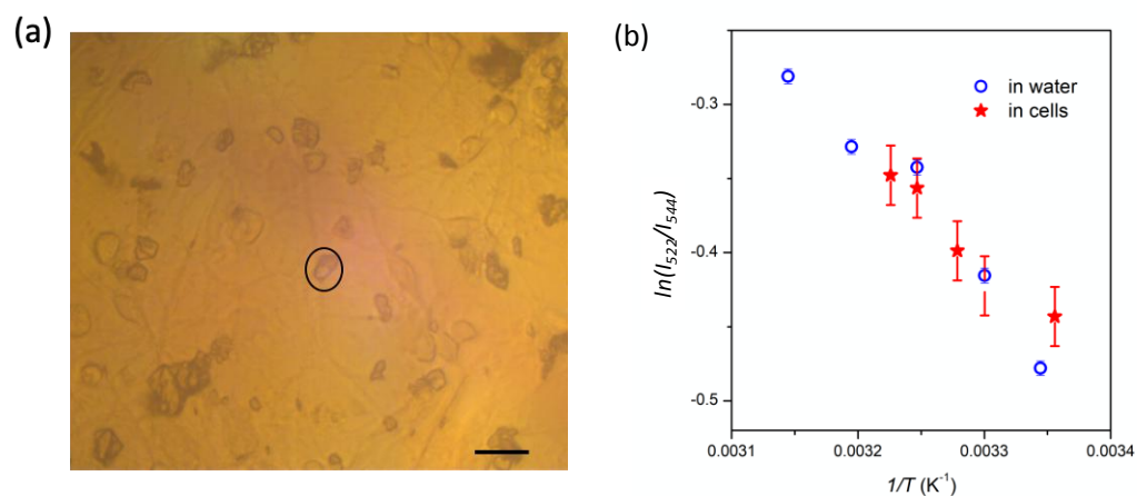
Figure 5. (a) Optical image of \text{Yb}^{3+},\text{Er}^{3+} -doped \alpha\text{-La}(\text{IO}_3)_3 nanocrystals loaded onto neuronal cells with a concentration of 0.1 mg/mL, in water (Scale bar: 12 \mu\text{m} ). (b) Evolution of LIR of the nanocrystals adsorbed on neurons as a function of temperature.
