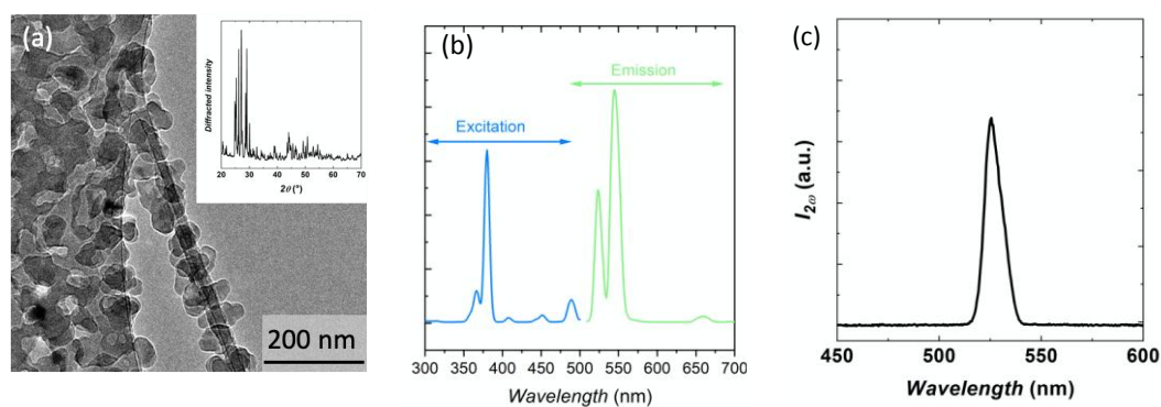
Figure 1. (a) Low-temperature TEM image of Yb 3+ ,Er 3+ -doped \alpha -La(IO 3 ) 3 nanocrystals. The inset shows the powder X-ray diffraction pattern associated with these nanocrystals. (b) Room-temperature PL and PL excitation spectra of Yb 3+ ,Er 3+ -doped \alpha -La(IO 3 ) 3 nanocrystals. The PL spectrum was recorded under a 380 nm excitation, whereas the PL excitation was recorded while monitoring the emission at 545 nm spectrum. (c) Second Harmonic Scattering signal from Yb 3+ ,Er 3+ -doped \alpha -La(IO 3 ) 3 nanocrystals in ethylene glycol under a 1064-nm excitation.
