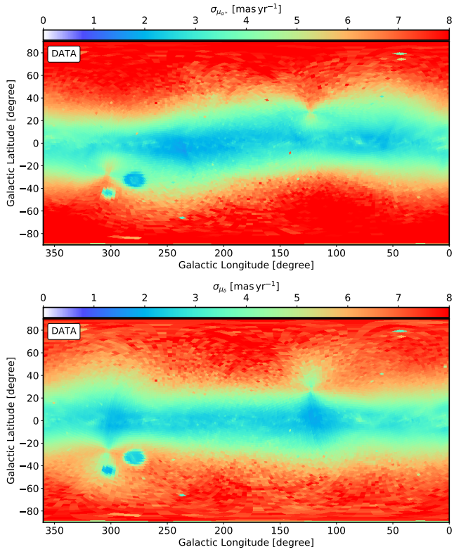
Fig. A.2. Dispersion in proper motion of the stars selected according to the criteria set in Sect. 2 as a function of position in the sky. Top: Proper motion in right ascension. Bottom: Same but in declination.
