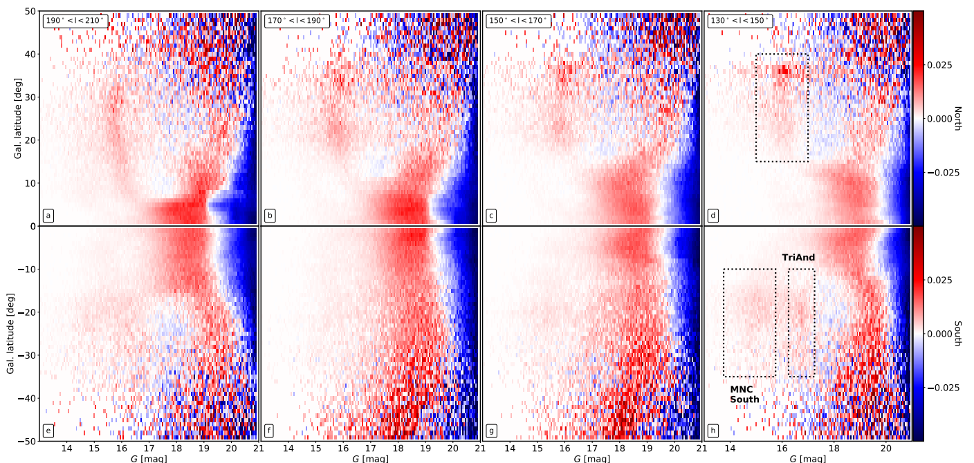
Fig. 8. Differences between the data and the mock in the plane of apparent magnitude against Galactic latitude of counts in the peak stars, for different bins in longitude. The plots are obtained by subtracting the counts from the top and bottoms panels of Fig. 7, and similar panels for the other ranges of longitude, which had been previously normalised by bins of latitude. From right to left: 130^\circ < l < 150^\circ , 150^\circ < l < 170^\circ , 170^\circ < l < 190^\circ , and 190^\circ < l < 210^\circ .
