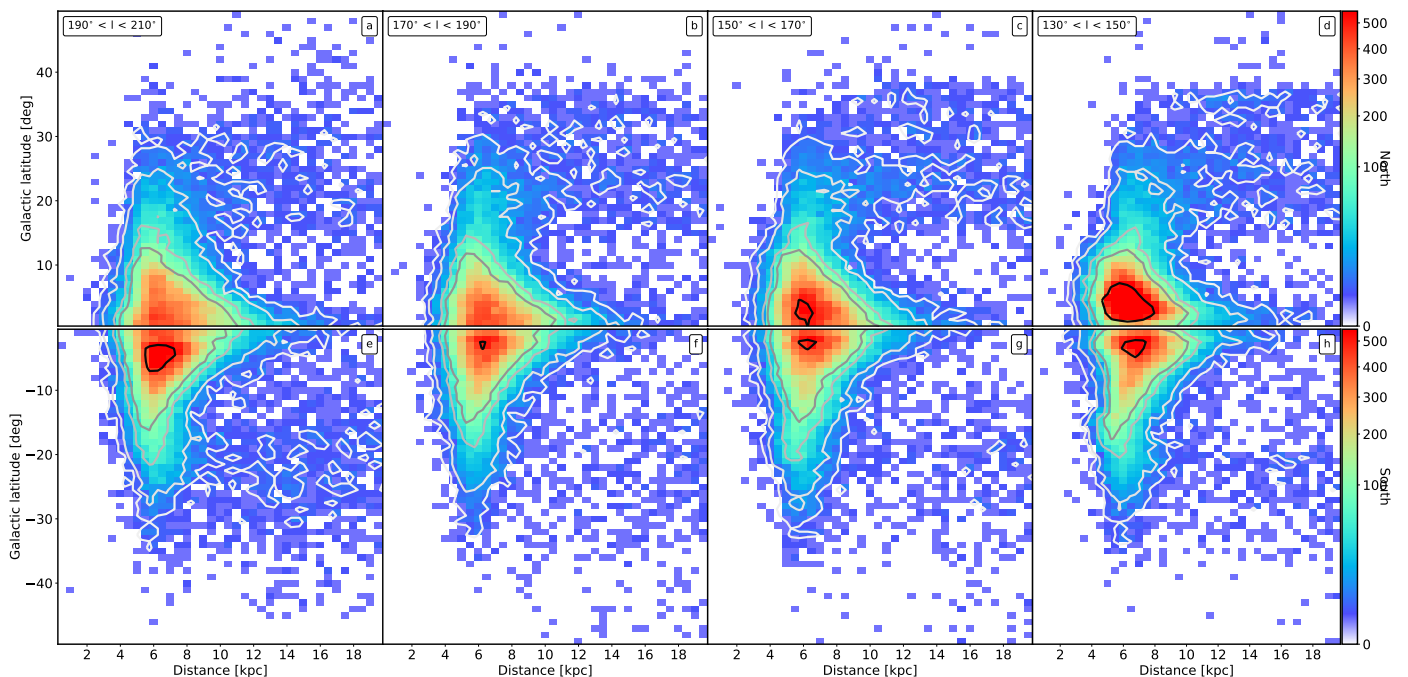
Fig. 10. Distance from StarHorse as a function of Galactic latitude for different slices in Galactic longitude, only for the giants stars within the peak. From right to left: 130^\circ < l < 150^\circ , 150^\circ < l < 170^\circ , 170^\circ < l < 190^\circ , and 190^\circ < l < 210^\circ .
