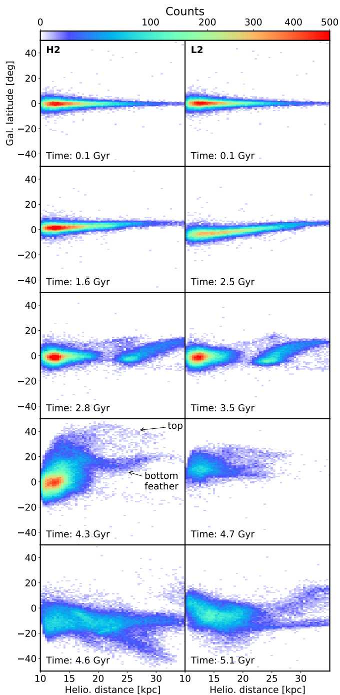
Fig. 11. Heliocentric distance against Galactic latitude for different snapshots of the simulations by Laporte et al. (2018). On the left, the H2 simulation and, on the right, the L2. In both cases, the Sun has been placed at (x=-8 \text{ kpc}, y=0 \text{ kpc}) . The stars shown in each panel correspond to those in slices of Galactic longitude 120^\circ < l < 240^\circ . The snapshot at 4.3 Gyr for H2 corresponds to the one where ACS- and MNC-like structures (top and bottom feathers, respectively) have been reported in Laporte et al. (2019a).
