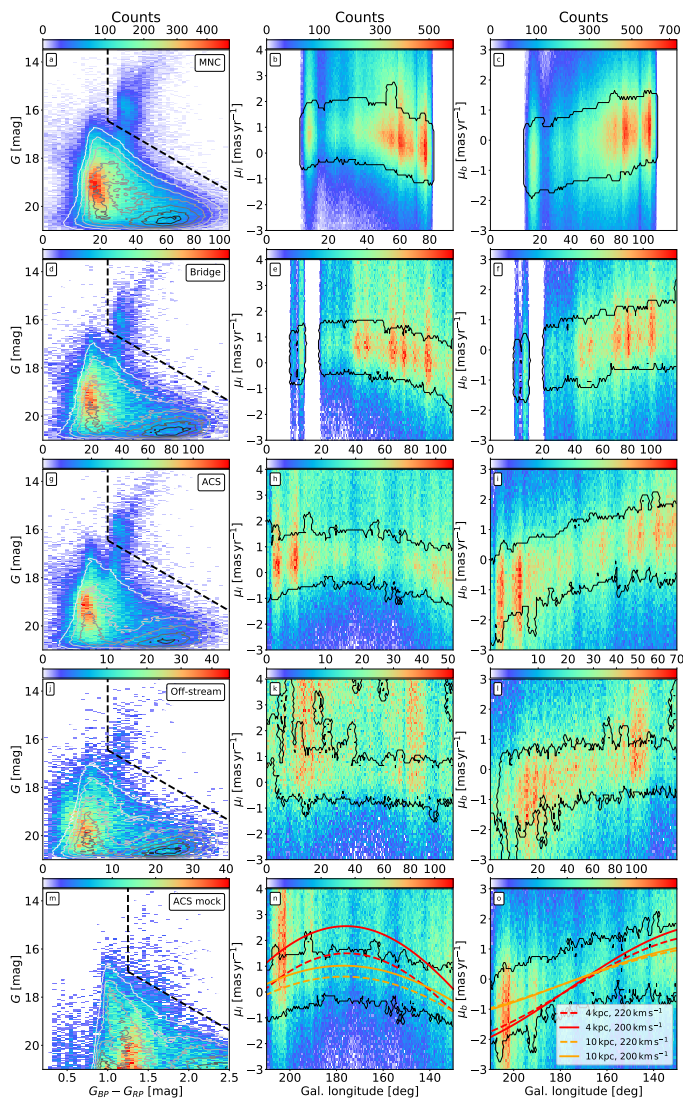
Fig. 5. CMD (left) and proper motion trends with Galactic longitude in \mu_l (middle) and \mu_b (right) of each structure. The CMDs contain the histogram of the stars within the highest intensity proper motion peaks (peak stars) with grey contours on top that represent the CMDs of all the stars in the region. The black dashed lines represent our selection of Giant stars. The proper motion maps contain all the stars in the region, and the black line is the zero-contour of the peak stars, that is, the stars that fall within the highest intensity proper motion peak of their HEALpix. First row: MNC. Second row: Bridge between MNC and ACS. Third row: ACS. Forth row: above ACS. Fifth row: Same region as ACS but for the mock particles, selecting the stars for the CMD according to the contours of panels h and i . In the bottom panel we also include the proper motions expected from a structure 30^\circ above the plane at a given distance, 4 (red) or 10 (orange) kpc, rotating at a given velocity, 200 (solid) or 220 (dashed) \text{km s}^{-1} , but with no radial or vertical velocity.
