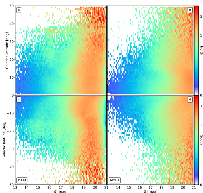
Fig. 7. Apparent magnitude as a function of Galactic latitude for the stars in the peaks with 130^{\circ} < l < 150^{\circ} . The histograms are normalised such the sum of all pixels in a given bin of b adds up to unity. A conspicuous overdensity of stars can be clearly seen appearing at G \sim 16 mag and extending from 15^{\circ} < b < 40^{\circ} . Left: Data. Right: Mock.
