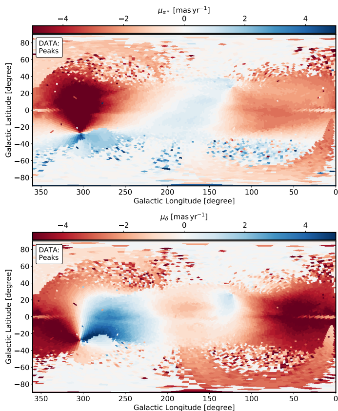
Fig. 3. Proper motion coordinates of the dominant peak at each HEALpix. Top: Proper motion in right ascension. Bottom: Same but in declination. Conspicuous stream-like patterns crossing the entire Celestial sphere can be appreciated, one of which is Sgr (bottom right to top left) and the other corresponds to the quasars (bottom left to top right).
