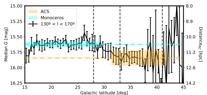
Fig. 9. Apparent magnitude of giants peak stars in the anticentre region ( 130^\circ < l < 170^\circ ) as a function of Galactic latitude, after correcting for extinction (see text). The error bars denote the 1\sigma uncertainty on the median computed as \sigma \sqrt{\frac{\pi}{2N}} , where \sigma is the standard deviation of the apparent magnitude in the bin. Vertical lines represent the approximate limits of each structure in that range of Galactic longitudes (see Fig. 4), and the right axis represents the distance to a RC star with the apparent magnitude shown in the left axis. The horizontal lines correspond to the median G magnitude for the giants peak stars within MNC (cyan) and ACS (orange). The shaded areas contain the \pm 3\sigma interval of uncertainty on the median and they extend from the minimum to the maximum latitude of the peak stars within each patch (the vertical dashed lines serve only as an orientation). As can be seen, the ACS is fainter than MNC and this translates to a difference in distance of \sim 1 kpc.
