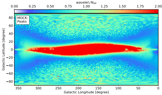
Fig. B.1. Relative intensity of the dominant structure in the proper motion plane of each HEALpix for the mock catalogue.
