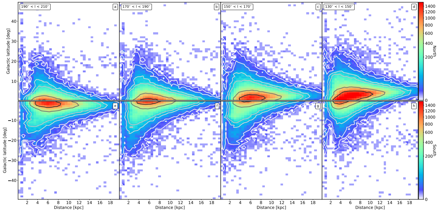
Fig. B.3. Same as Fig. 10 but for the particles in the mock catalogue that fall inside the peaks detected in the data.
