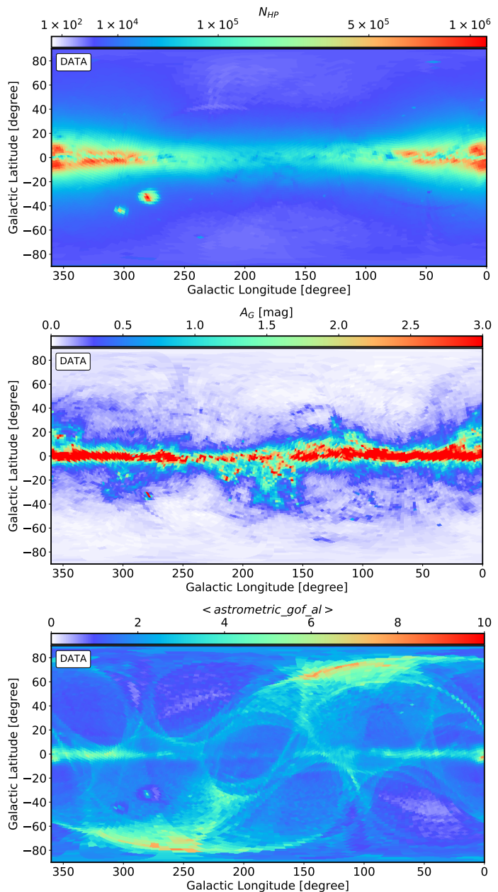
Fig. 2. Top: Number of stars in each HEALpix that fulfil the selection described in Sect. 2. Middle: Absorption at infinite in the G band at each HEALpix, obtained from the Schlegel et al. (1998) maps with the re-calibration by Schlafly & Finkbeiner (2011) and using the mean G_{BP} - G_{RP} colour in the HEALpix together with the transformations described in Appendix A of Ramos et al. (2020). Bottom: Average astrometric_gof_al at each HEALpix (see Appendix A).
