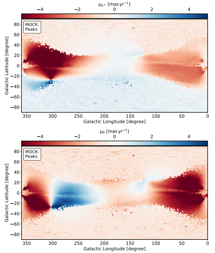
Fig. B.2. Same as Fig. 3 but for the mock.
