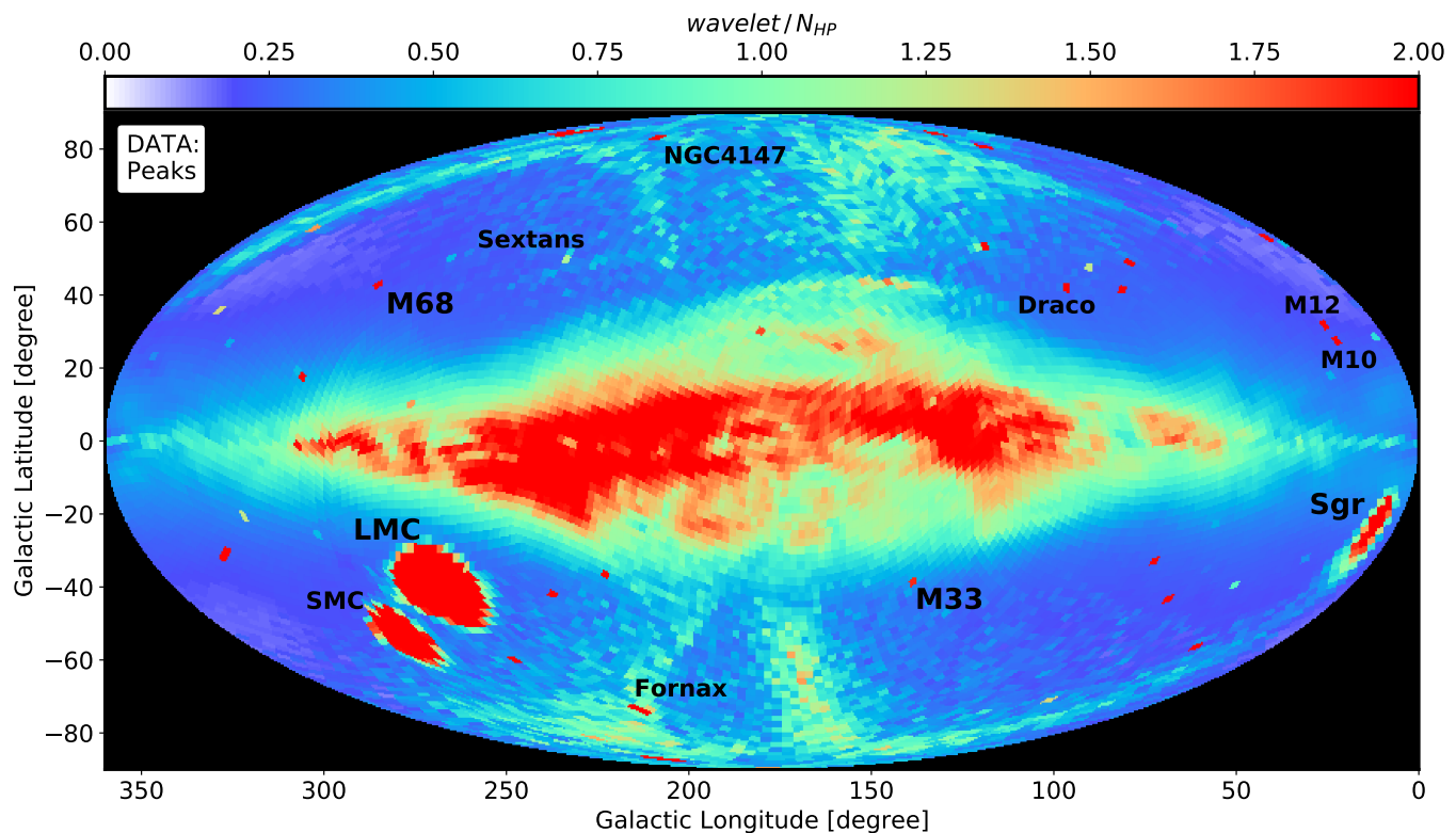
Fig. 1. Mollweide projection of the relative intensity of the dominant structure in the proper motion plane at each HEALpix. By showing only the most significant kinematic overdensity and normalising to the number of stars in the HEALpix, a large number of structures become visible: the Sgr stream, tens of globular clusters and an intricate anticentre. We have labelled some of most relevant ones.
