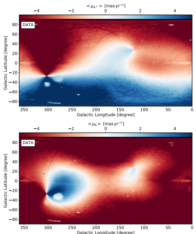
Fig. A.1. Average proper motion of the stars selected according to the criteria set in Sect. 2 as a function of position in the sky. Top: Proper motion in right ascension. Bottom: Same but in declination. Only a few globular clusters, the Large Magellanic cloud and the most inner parts of the Sgr core are noticeable, as the rest of the field is dominated by the solar reflex (peculiar motion of the Sun and rotation of the Local Standard of Rest).
