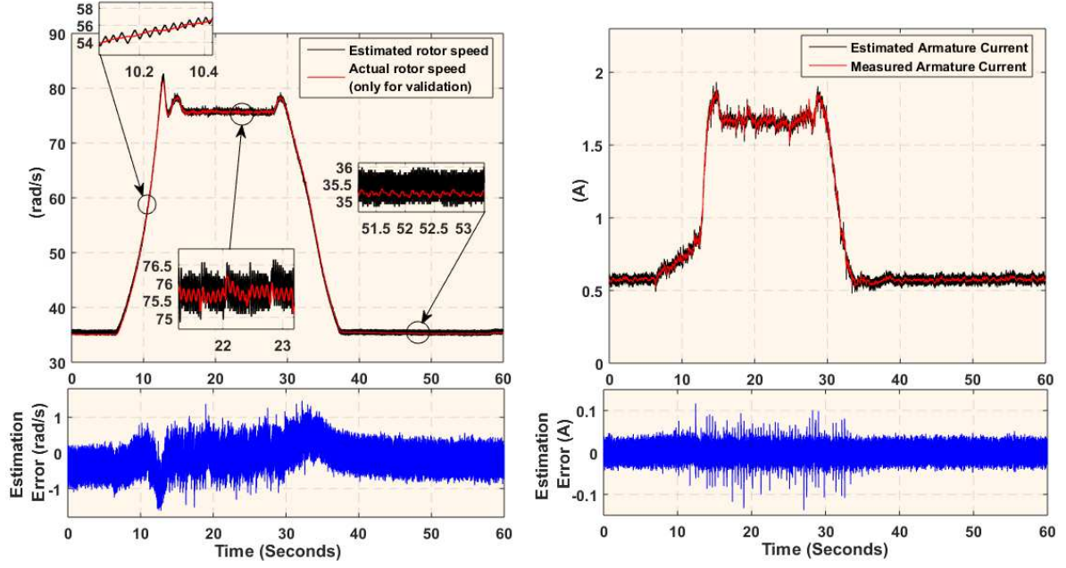
Fig.9 Experimental estimation performance under increasing and decreasing rotational speed profile.
