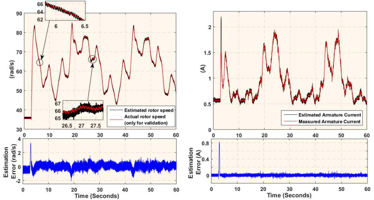
Fig.10 Experimental estimation performance under random rotational speed profile.
