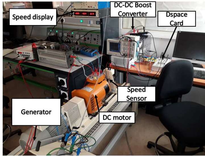
Fig.6. Experimental setup of the realized wind turbine emulator (WTE).
