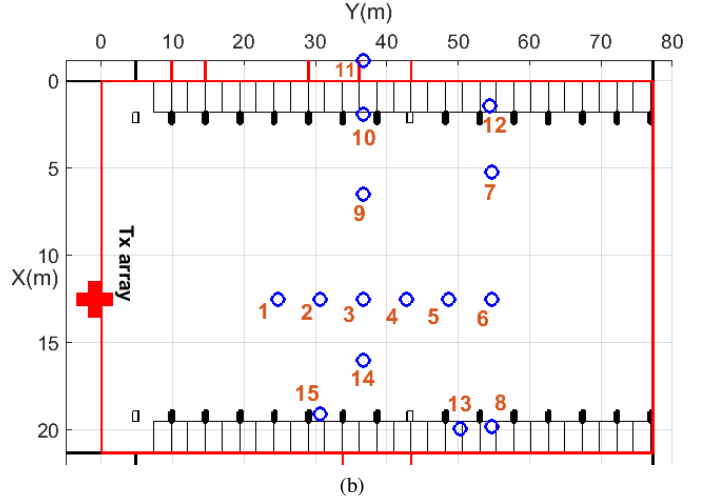
Fig. 1. a) Panoramic view of the industrial hall (Tx at the left side of the figure) and b) Top view showing the positions of Tx and those of the various UEs.
