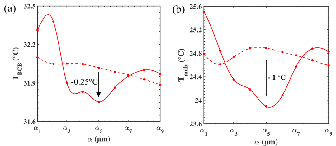
Figure 6. Evolution of (a) the temperature of the membrane T_{\text{BCB}} = T_1 = T_2 and (b) the ambient temperature as a function of the scaling factor \alpha_i for a structured (solid lines) and non-structured (dashed lines) membrane.
