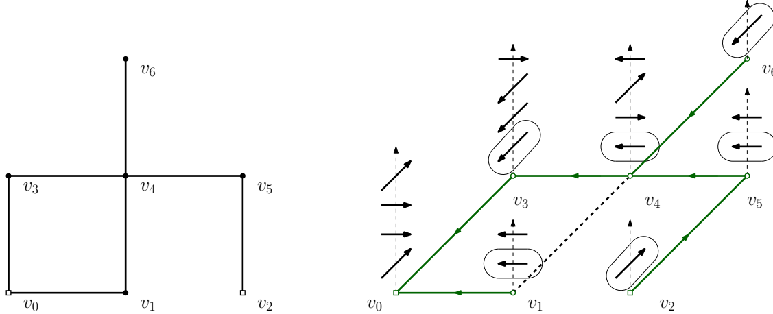
Figure 1: Left: graph G , where the walk w = v_0 v_3 v_0 v_1 v_0 v_1 v_0 v_3 v_0 v_3 v_4 v_5 v_4 v_6 v_4 v_3 v_4 v_5 v_2 is performed. Right: Heap associated to the path w ; for example, H_{v_3} = [(v_3, v_0), (v_3, v_0), (v_3, v_0), (v_3, v_4)] . To read the steps of w in the heap, follow the edges from top to bottom to form \overleftarrow{w} , then transform \overleftarrow{w} into w . The steps used to construct the tree are circled
