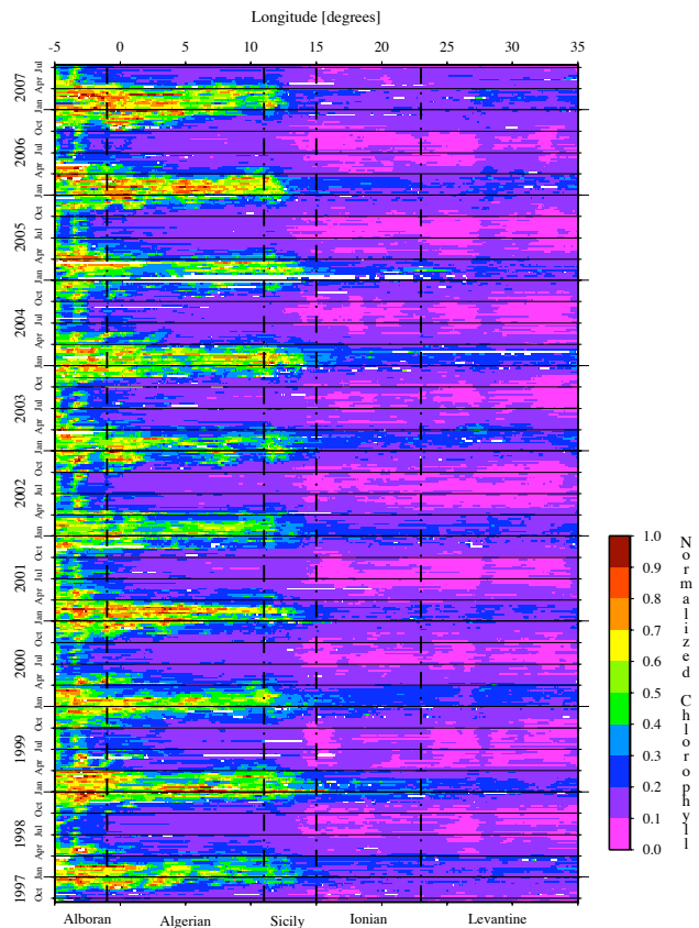
Fig. 2. Hoemoeller diagram on the West-East transect of Normalized Chlorophyll concentration (see Fig. 1 for the geographical position of the transect). Normalized Chlorophyll is calculated normalizing the values along the transect by the maximum value of the transect.
