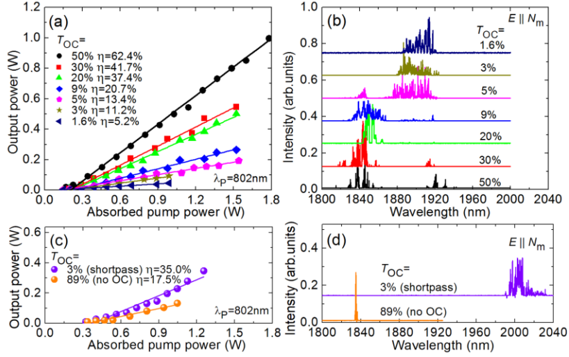
Fig. 9. Continuous-wave Tm channel WG laser with conventional pumping ( \lambda_p = 802 nm): (a,c) input-output dependencies, \eta – slope efficiency; (b,d) typical laser emission spectra, P_{abs} = 1 W. The laser polarization is E \parallel N_m .
