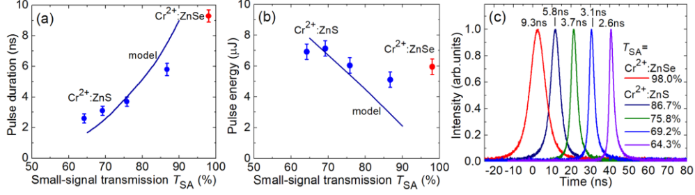
Fig. 19. Tm channel WG laser passively Q-switched by Cr^{2+}:ZnS and Cr^{2+}:ZnSe SAs with different small-signal transmission T_{SA} : (a) pulse duration, (b) pulse energy and (c) the corresponding oscilloscope traces. Panels (a),(b): symbols – experimental data, curves – numerical modeling. T_{OC} = 50\% , P_{abs} = 0.8 W.
