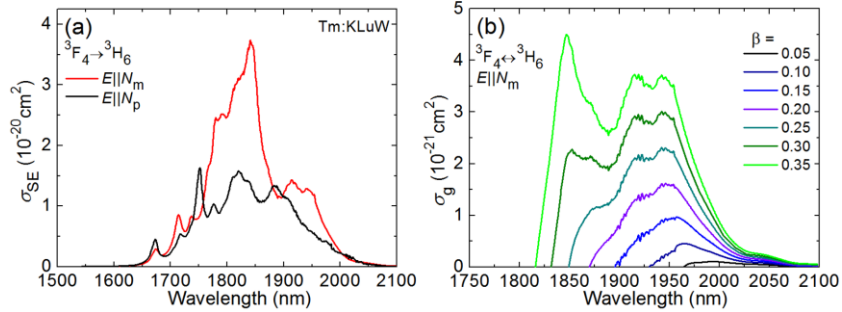
Fig. 10. Emission properties of Tm^{3+} ions in KLuW at \sim 2 \mu m (the {}^3F_4 \leftrightarrow {}^3H_6 transition): (a) stimulated-emission (SE) cross-sections, \sigma_{SE} , for light polarizations E \parallel N_m and E \parallel N_p ; (b) gain cross-sections, \sigma_g = \beta\sigma_{SE} - (1-\beta)\sigma_{abs} , for light polarization E \parallel N_m and various inversion ratios \beta = N_2({}^3F_4)/N_{Tm} , N_2 is the population of the upper laser level.
