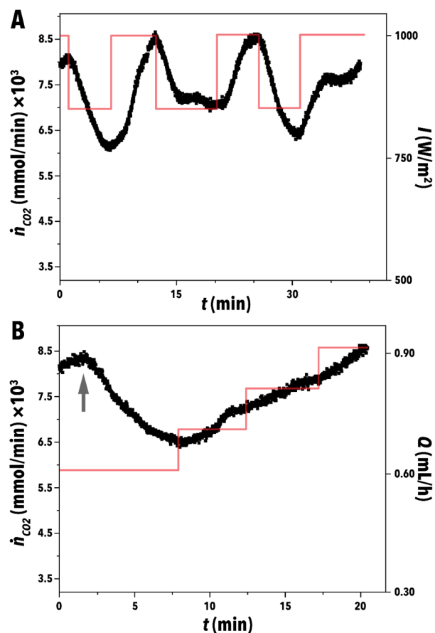
Figure 7. (A) Fluctuations in CO 2 release caused by variation in I between \sim 1000 W/m 2 and \sim 860 W/m 2 . (B) Proof-of-concept for feedforward control based on irradiance. CO 2 release is returned to its original value by varying the aqueous amine feed flow rate.
