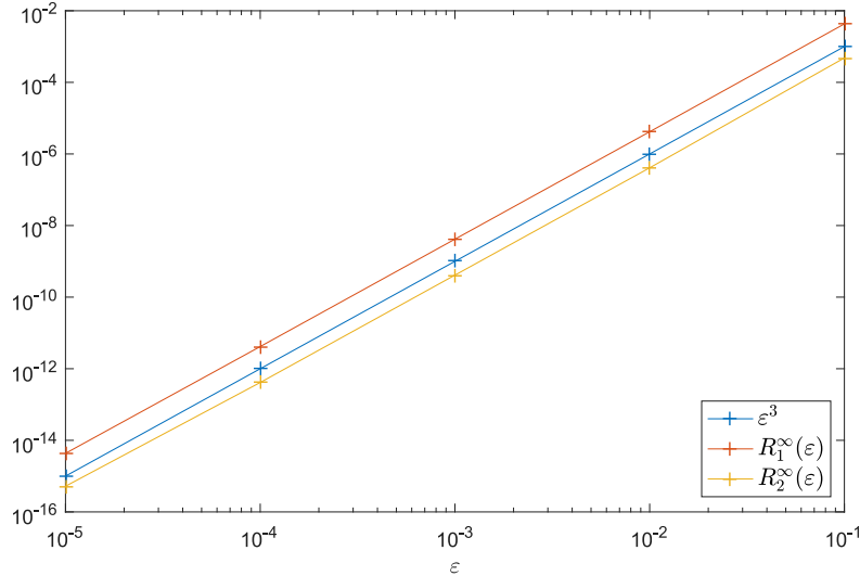
FIGURE 5. The residues R_1^\infty and R_2^\infty as a function of \epsilon .
