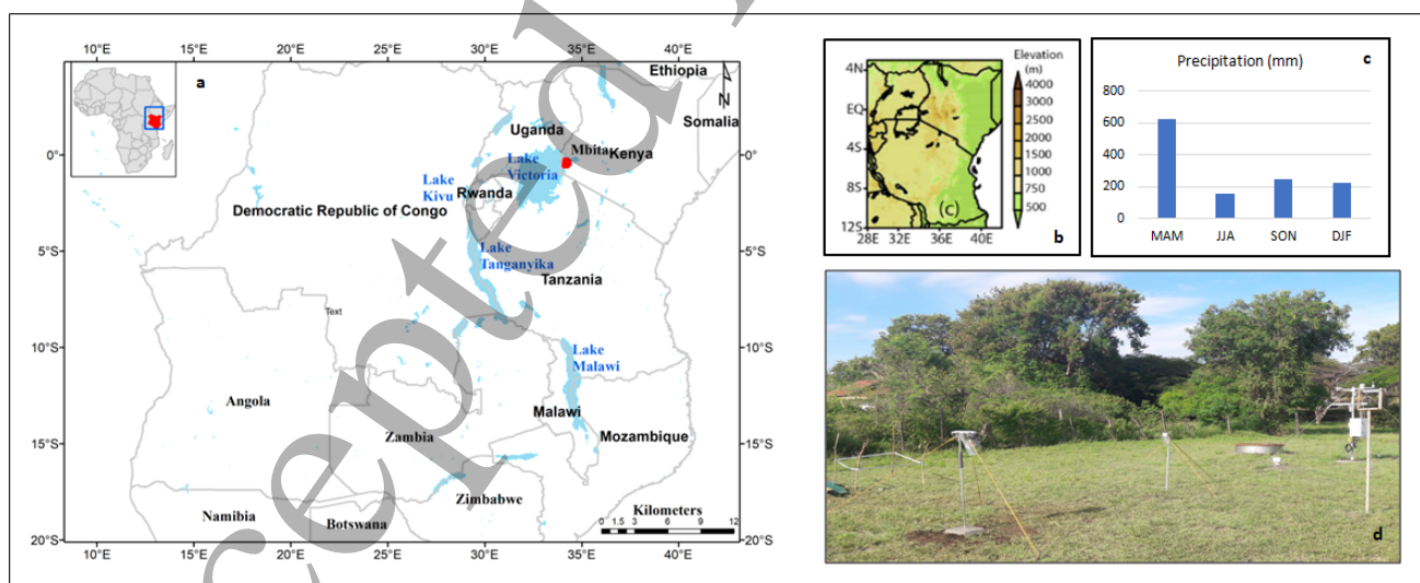
56 23 Figure 1: (a) Map of the study area on the African Continent (shown top left in the insert). Location of the site of 57 24 Mbita (red circle). Blue labeling represents the major African lakes and ocean. (b) Topographic map within the study 58 25 domain. (c) Mean precipitation at Mbita according to seasonal climatology for the period 1985-2019 with March 59 26 60 27
