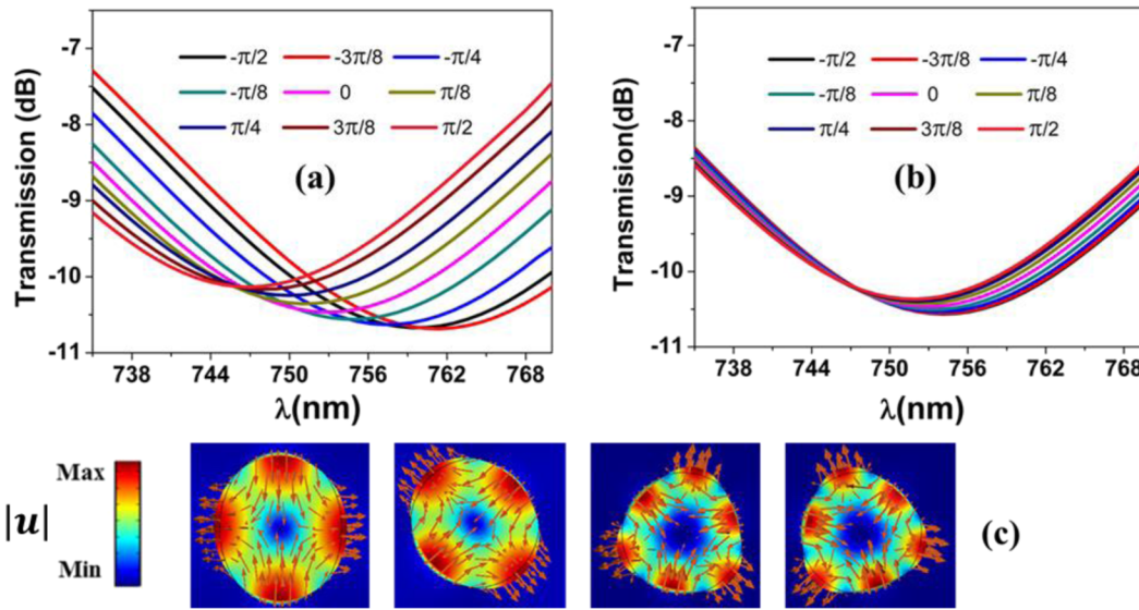
FIG. 5. Evolution of the transmission spectra for different values of the elastic phase for the two elastic modes: (a) mode \alpha and (b) mode \beta . (c) Norm of the displacement field distribution [\mathbf{u} = (u_x, u_y, u_z)] for \alpha, \beta, \gamma, and \delta modes at the \Gamma point (color map shows the norm of displacement field |\mathbf{u}| ; red arrows represents the real part of \mathbf{u} ).
