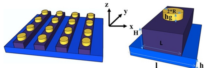
FIG. 1. Sketch of the structure with the unit cell and corresponding geometrical parameters.
