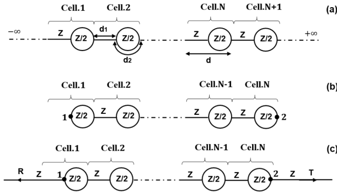
FIG. 12. (a) The infinite periodic structure made of a wire of length d_1 and a loop formed out by two wires, each of length d_2 , d = d_1 + d_2 is the period of the structure. (b) The finite periodic structure containing N cells with loop termination on both sides. (c) The finite periodic structure inserted between two semi-infinite wires.
