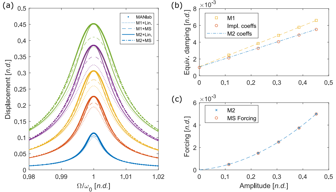
Figure 1: Validation of the identification methods, without geometric nonlinearities.
