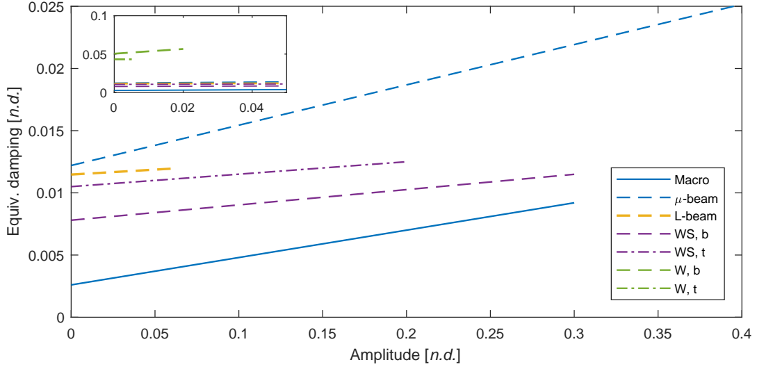
Figure 11: Reconstructed equivalent damping \xi_{eq} , computed with the values identified using M2a (cantilever beams) and M2b (beam assemblies) for the tested modes.
