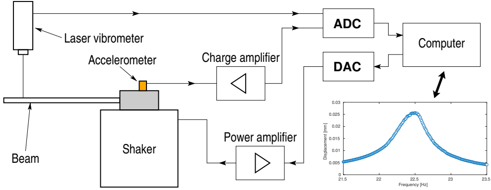
Figure 4: Experimental setup for the measurement of the frequency response curves.
