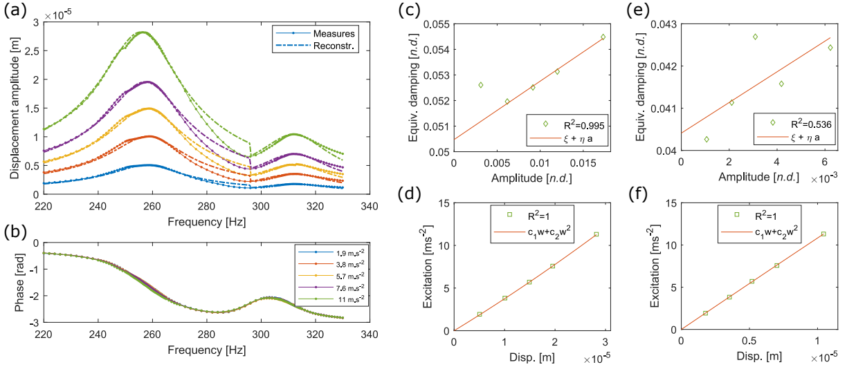
Figure 10: Measurement, identification and reconstruction for the "true" wing (bending and twisting modes).
