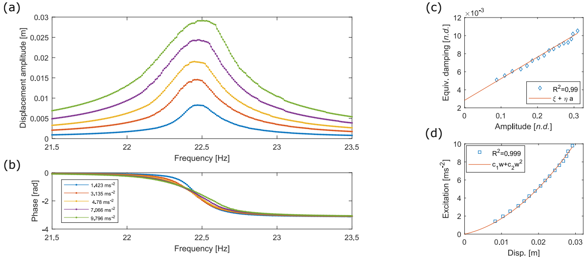
Figure 5: Damping coefficients extraction for the ruler's first mode.
