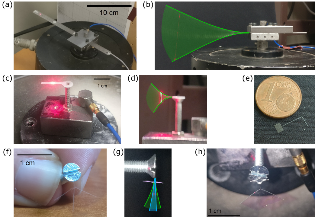
Figure 3: Photographs of tested specimens.
