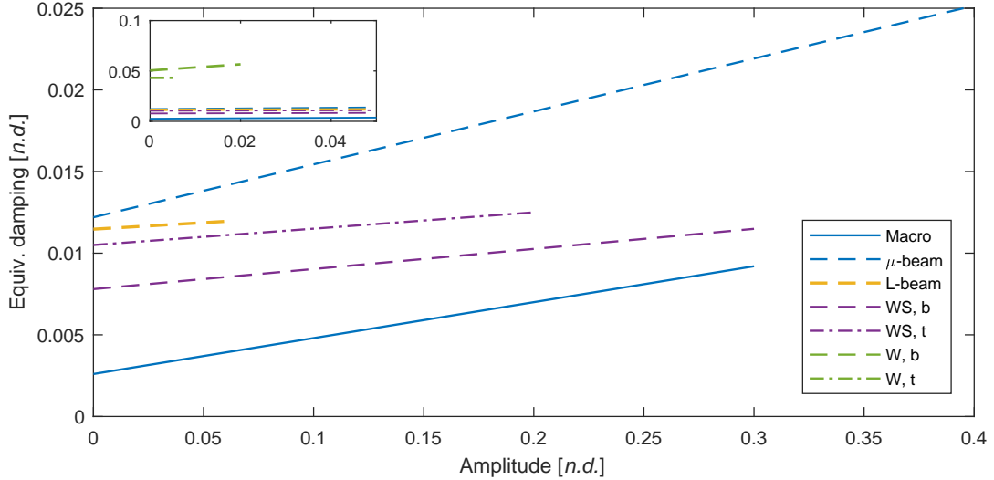
Figure 11: Reconstructed equivalent damping \xi_{eq} , computed with the values identified using M2a (cantilever beams) and M2b (beam assemblies) for the tested modes.
