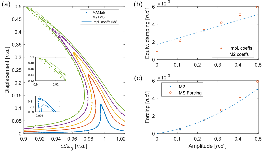
Figure 2: Validation of the second identification method, with geometric nonlinearities.
