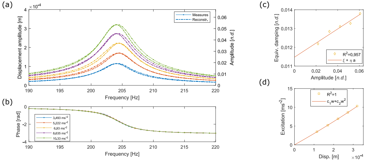
Figure 8: Measurement, identification and reconstruction for L-beam (mode 1).
