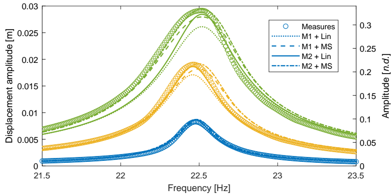
Figure 6: Experimental validation of identification methods and models for a steel ruler (filt).
