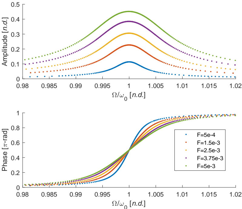
Figure 12: Simulated frequency responses with MANlab
