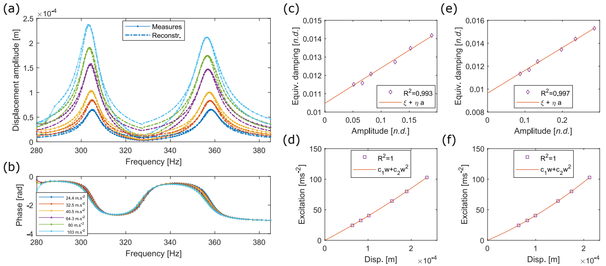
Figure 9: Measurement, identification and reconstruction for the Wing skeleton (bending and twisting modes).
