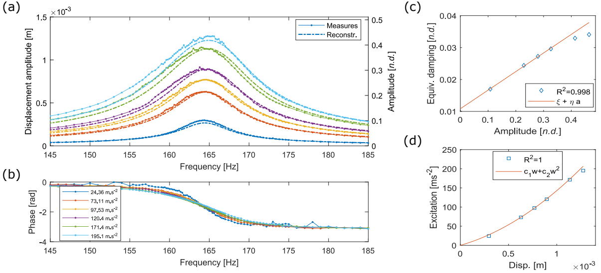
Figure 7: Measurement, identification and reconstruction for \mu -beam (mode 1).
