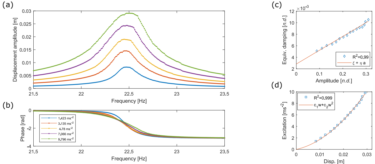
Figure 5: Damping coefficients extraction for the ruler's first mode.
