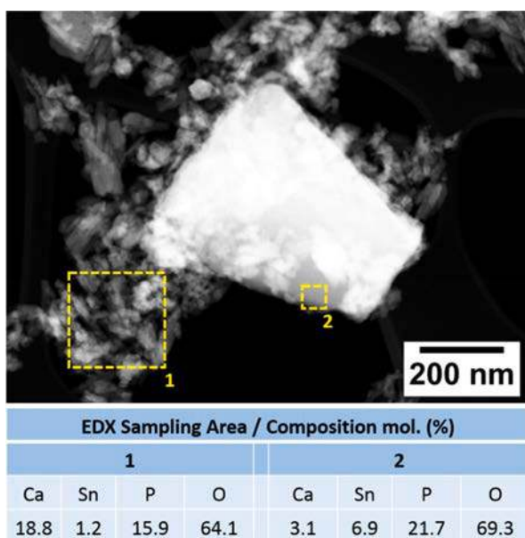
Fig. 3. HAADF-STEM micrograph of Sn7.5/HAP sol sample and EDX semi-quantitative analysis of the areas selected on the image.
