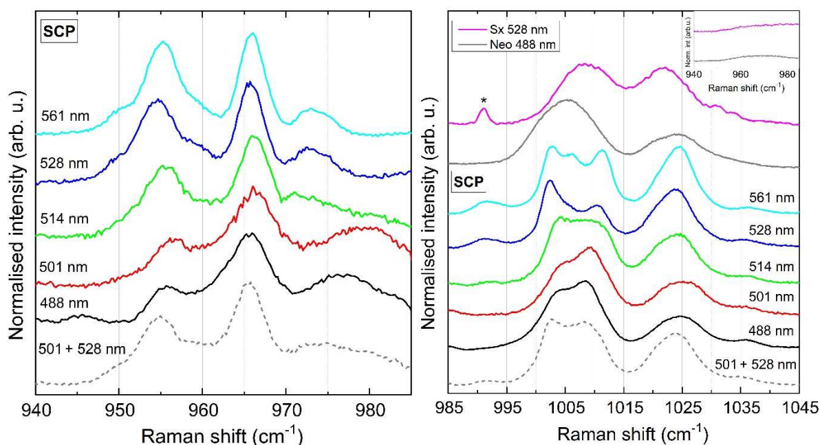
Fig. 4. Resonance Raman spectra at 77 K in \nu_4 (left) and \nu_3 (right) regions of SCP, excited at 488.0, 501.7, 514.5, 528.7 and 561.0 nm. Also shown is the sum between 501.7 nm and 0.8 \times 528.7 nm ( \nu_1 -normalised spectra; dashed lines). Top spectra on the right: Sx and Neo in pyridine, excited at 528.7 and 488 nm, respectively; Inset: \nu_4 region of these spectra. *solvent band
