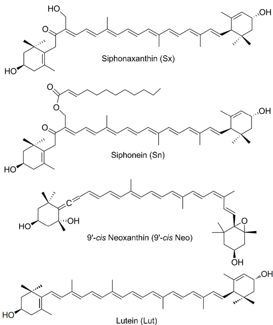
Fig. 1. Molecular structures of carotenoids siphonaxanthin and siphonein. Neoxanthin and lutein are shown for comparison.
