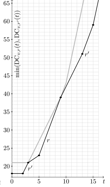
Figure 6: \min(DC_{v,r}(t), DC_{v,r'}(t))
