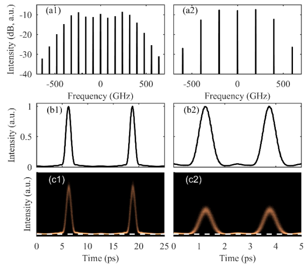
Fig. 3. (a) Spectral and (b) temporal intensity profiles after spectral components cancellation. (c) is the temporal profile recorded in the persistent mode. Panels (1) deal with a repetition rate of 80 GHz whereas panels (2) are obtained at 200 GHz.
