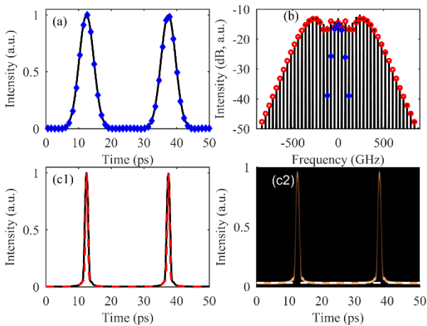
Fig. 2. (a) Temporal intensity profiles recorded on the optical sampling oscilloscope after the first linear shaping (solid line) are compared with the theoretical shape of the Besselon (blue diamonds). (b) Optical spectrum after modulation (blue diamonds) and after nonlinear propagation (black lines). Results of numerical simulations are plotted with red circles. (c1) Temporal intensity profiles after the nonlinear propagation and quadratic spectral phase. Results of numerical simulation (red dashed line) are compared with experimental results (black line). Panel (c2) is similar to (c1) but recorded in the persistent mode of the optical sampling oscilloscope.
